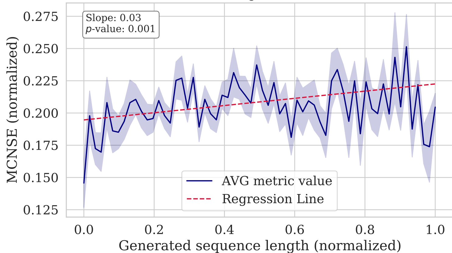
MCNSE vs. Length (WMT14 Fr-En)
