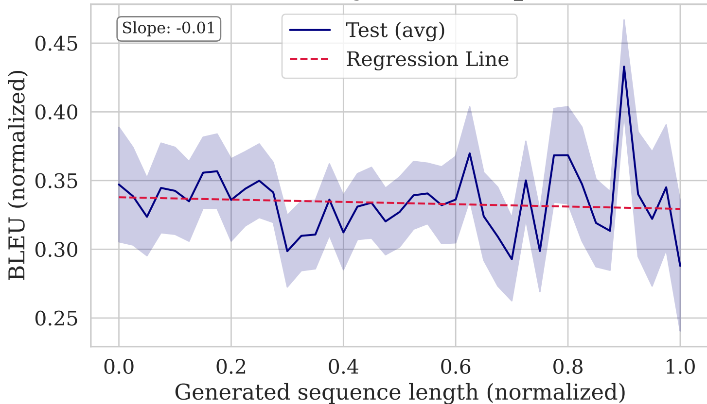
BLEU vs. Length (Test - wmt14_ruen)
