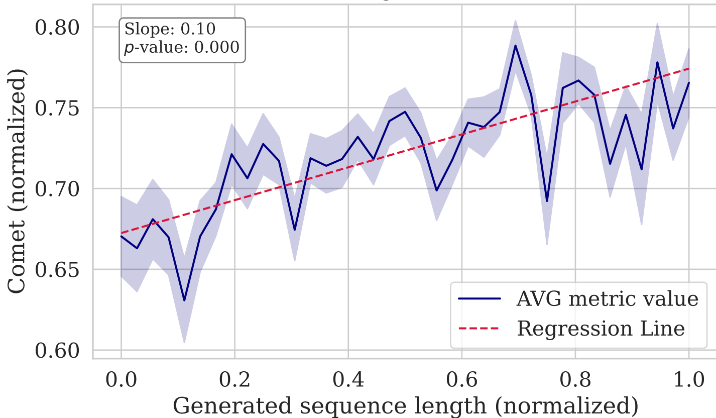
Comet vs. Length (WMT19 Fi-En)
