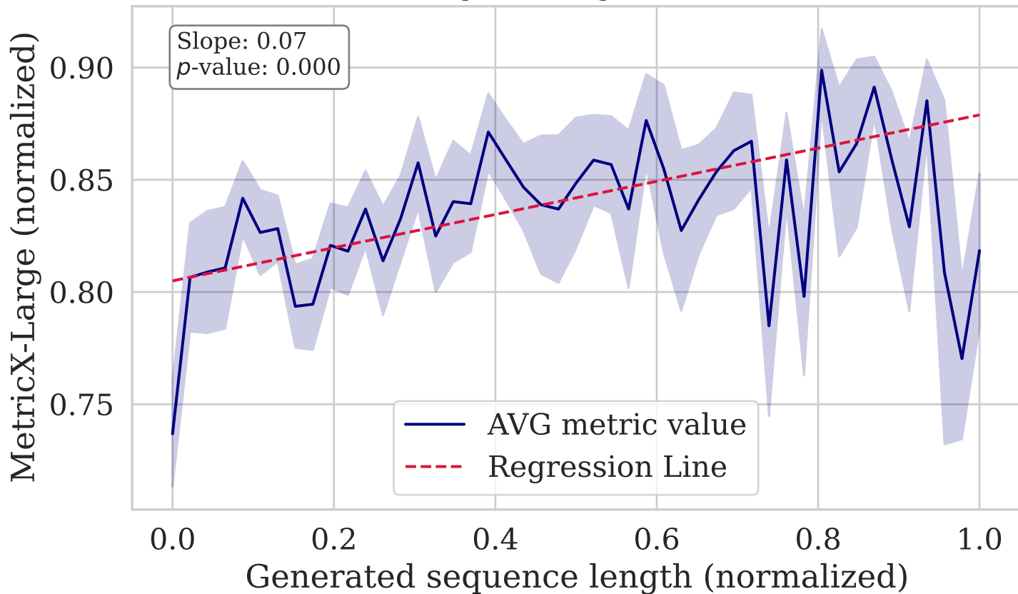
MetricX-Large vs. Length (WMT19 Fi-En)
