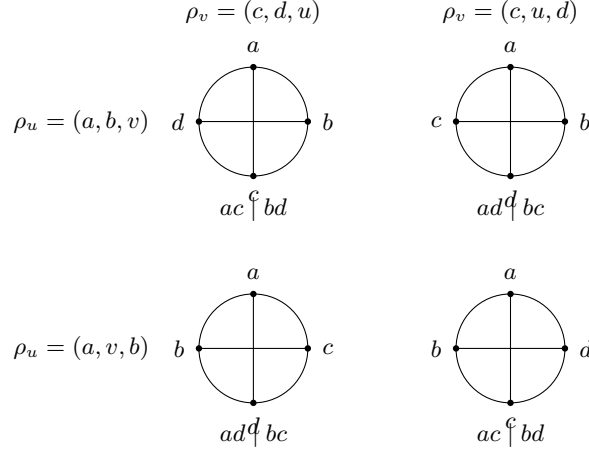
FIGURE 1. The four rotation choices for an induced quartet with true split ab \mid cd . In each circle the labels are shown in boundary order, and the two diameters join opposite positions; the split below the circle is therefore the crossing split.
