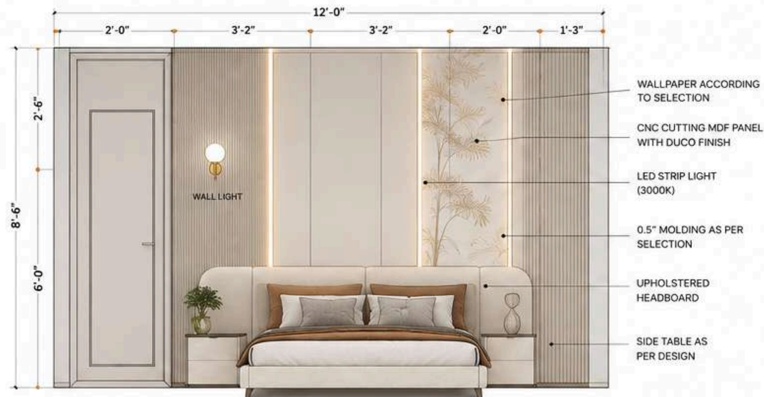
ELEVATION SCALE - 1:25
