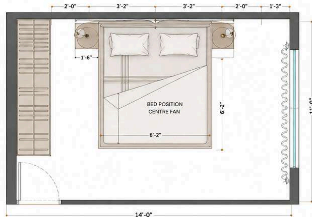
PLAN SCALE - 1:25
