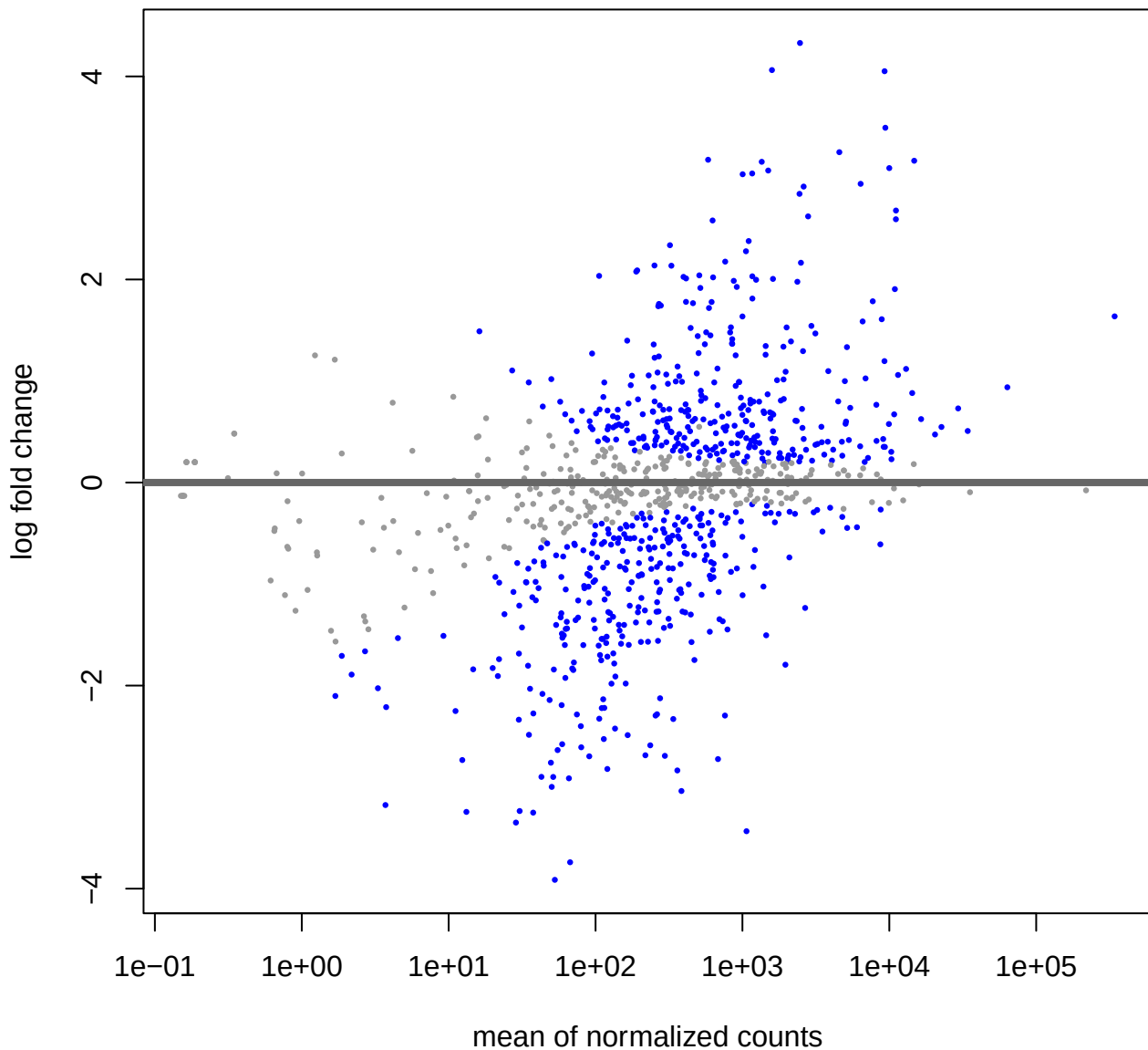
MA-plot for strain_type: wildtype vs mutant
