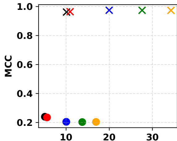
Chess
