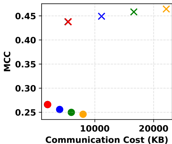
Connect-4
