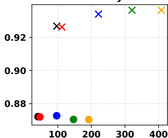
Nursery
