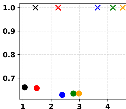
Car Evaluation
