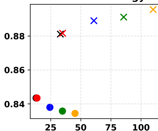
Nursery
