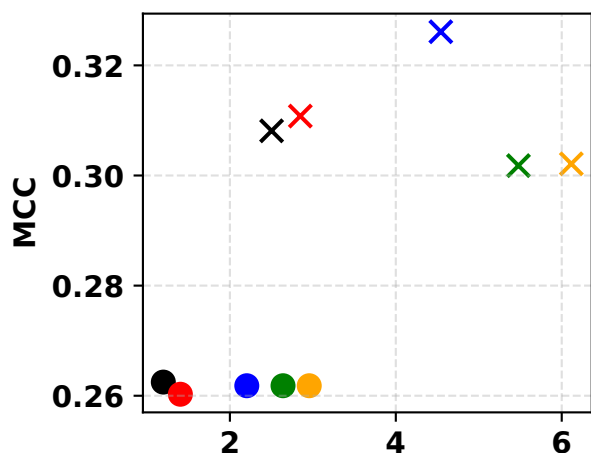
Tic-Tac-Toe
