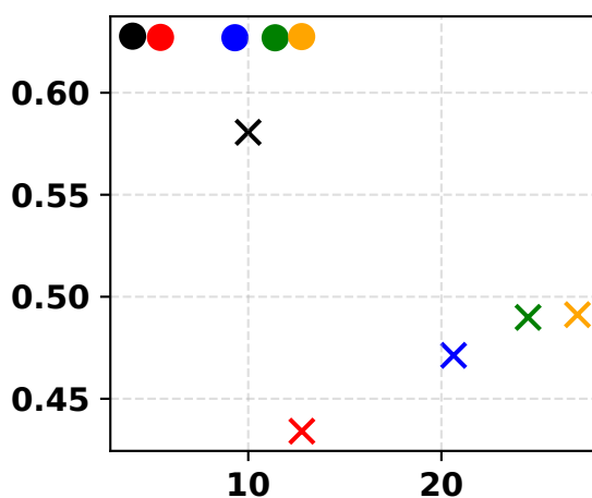
Mushroom
