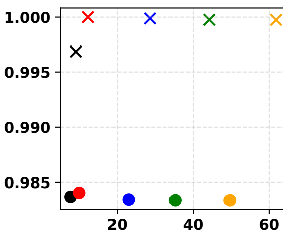
Mushroom
