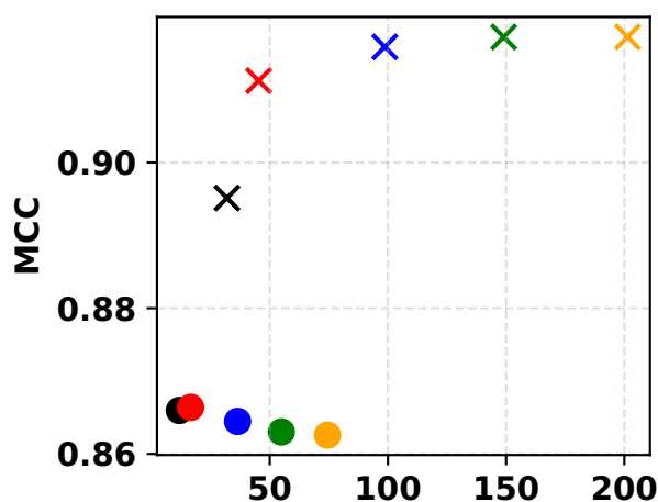
Connect-4
