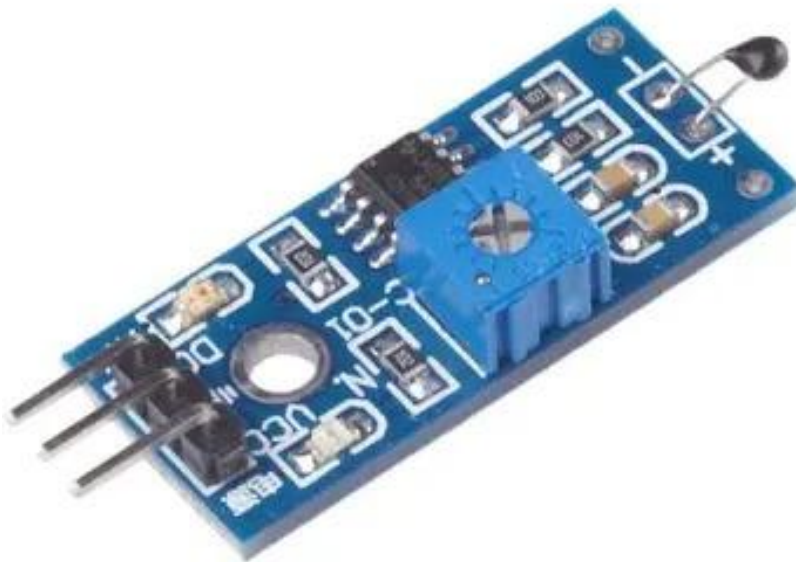
Figure 3: NTC Thermistor Sensor Module – with LM393 comparator and sensitivity potentiometer
