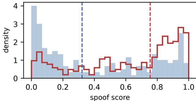
XLS-R / SIMPLESPEECH2 matched pooled median gap=0.433
