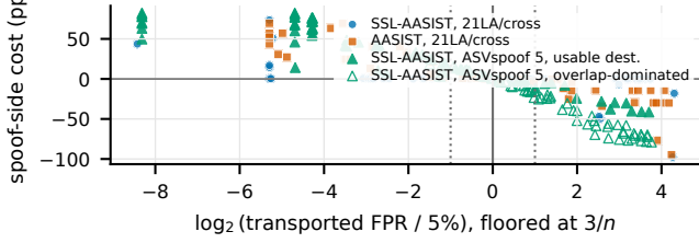
Fig. 1. Transported FPR against spoof-side cost. Each point is one deployment cell: severity \log_2(\max(\text{FPR}, 3/n)/5\%) (§4; dotted lines mark the 2\times bar) against mean FNR at the transported threshold minus FNR at the deployment-calibrated threshold, in points. Circles and squares are the 108 21LA and cross-corpus cells; triangles are the 132 ASVspoof 5 SSL-AASIST pairs, filled where the destination is usable (oracle FNR \leq 50\% for every source) and hollow where it is overlap-dominated. Conservative misses (left of centre) carry the positive costs.
