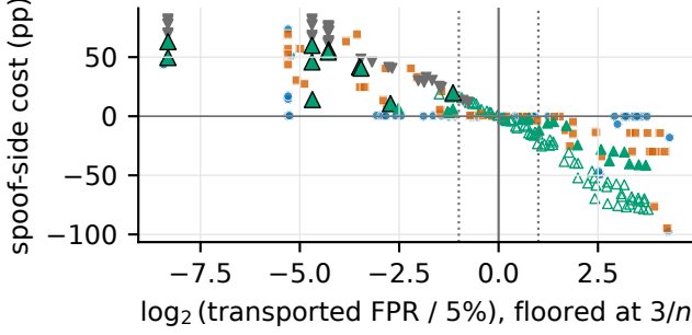
Fig. 1. Recoverable spoof loss by source usability. Each point is a deployment cell: x = \log_2(\max(\text{FPR}, 3/n)/5\%) (§4; dotted 2\times bars); y is mean transported FNR minus all-target-bona-fide oracle FNR (points). Blue circles/orange squares: 108 SSL-AASIST/AASIST 21LA and cross-corpus cells. Triangles: 132 ASVspoof 5 SSL-AASIST pairs; hollow, overlap-dominated destinations; filled, usable destinations (oracle FNR \leq 50\% for every source). Filled green upward/gray downward triangles distinguish 30 usable-source/36 weak-source transfers (same criterion); black outlines identify the 11 usable-source transfers exceeding +10 .
