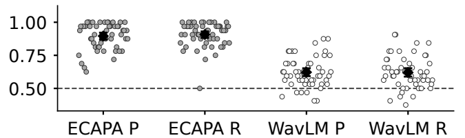
Fig. 2. Fixed-roster per-speaker attribution accuracy (54 dots/group; 32 comparisons per dot). Diamonds and bars are pooled points and 95% speaker-resampling stability intervals; the dashed line is chance. P/R: primary/reverse.
