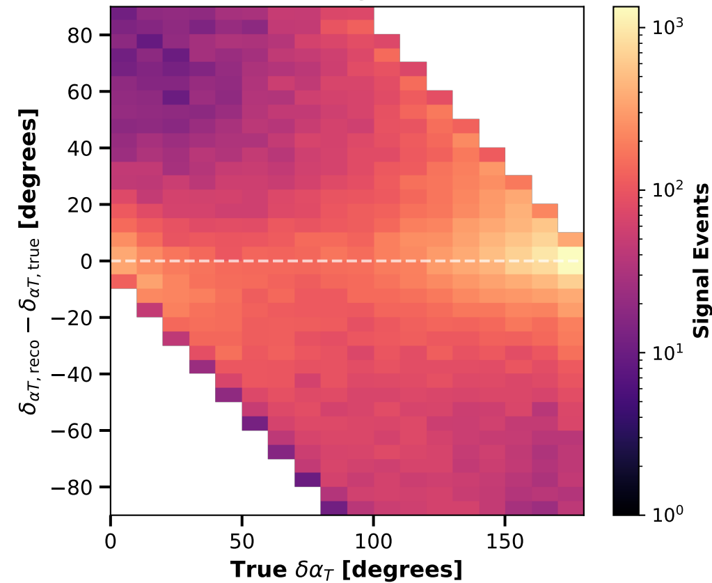
Exiting \mu^\pm
