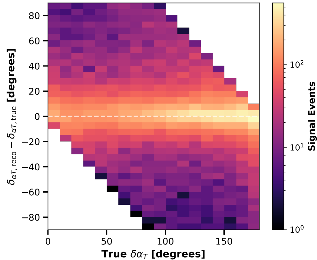
Contained \mu^\pm
