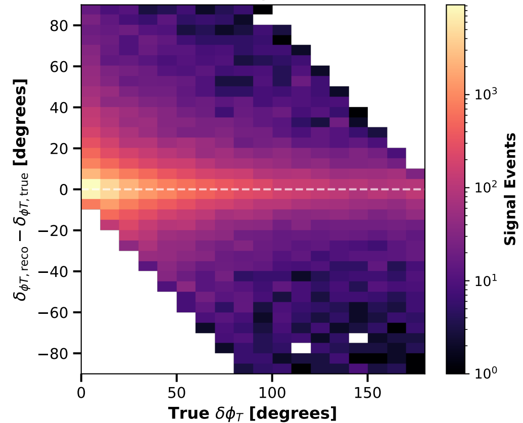
Exiting \mu^\pm
