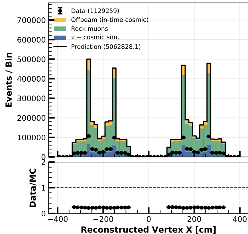
ICARUS • NuMI Data (10% Run 2) Work-in-Progress
