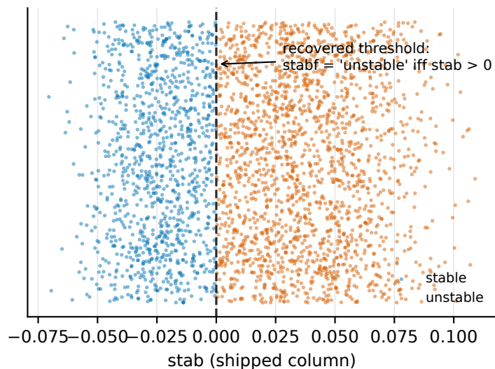
(a) Grid Stability: label = sign of shipped column
