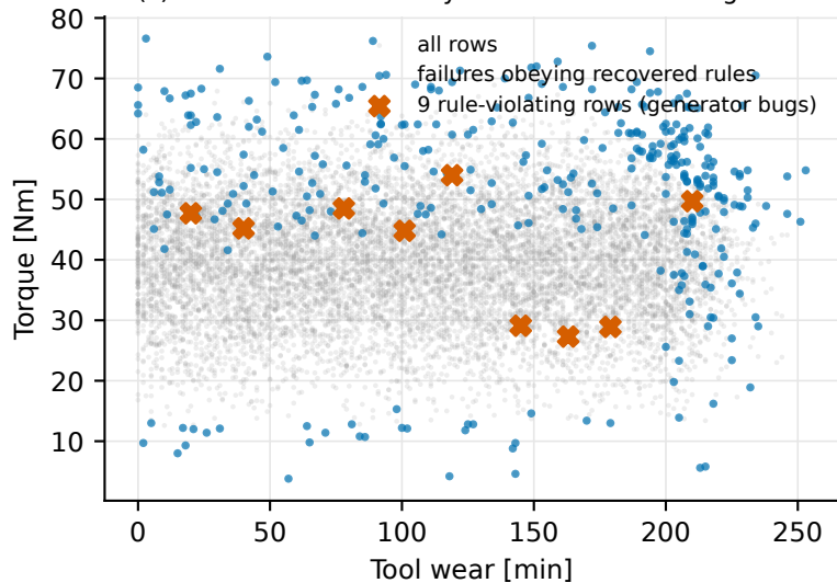
(c) AI4I 2020: rule fidelity 0.9991 isolates 9 bug rows
