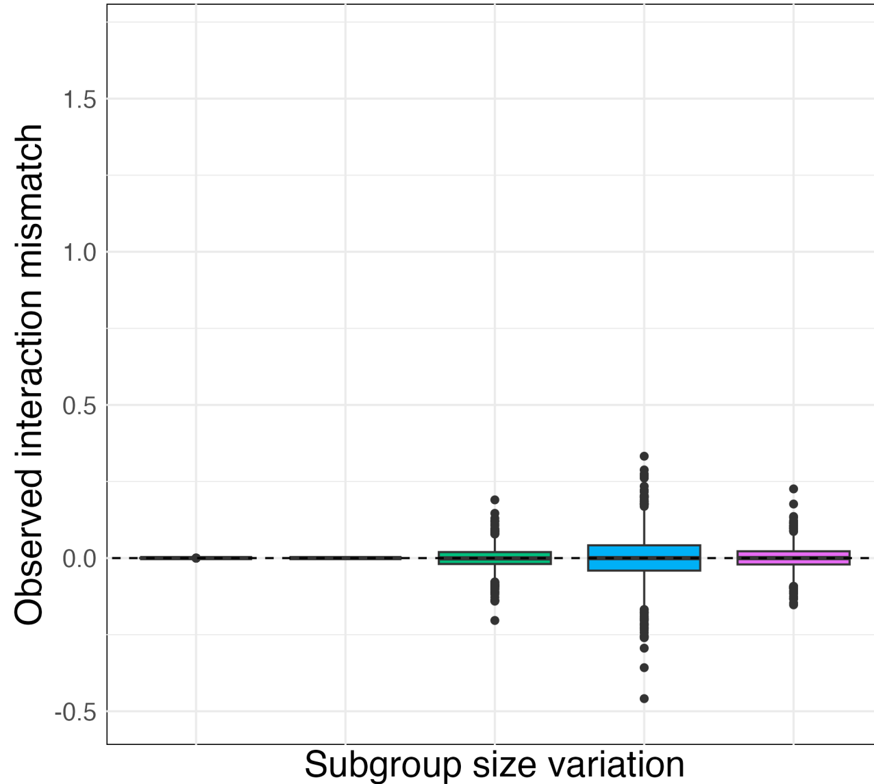
Noncollapsibility without confounding (no aggregation bias)
