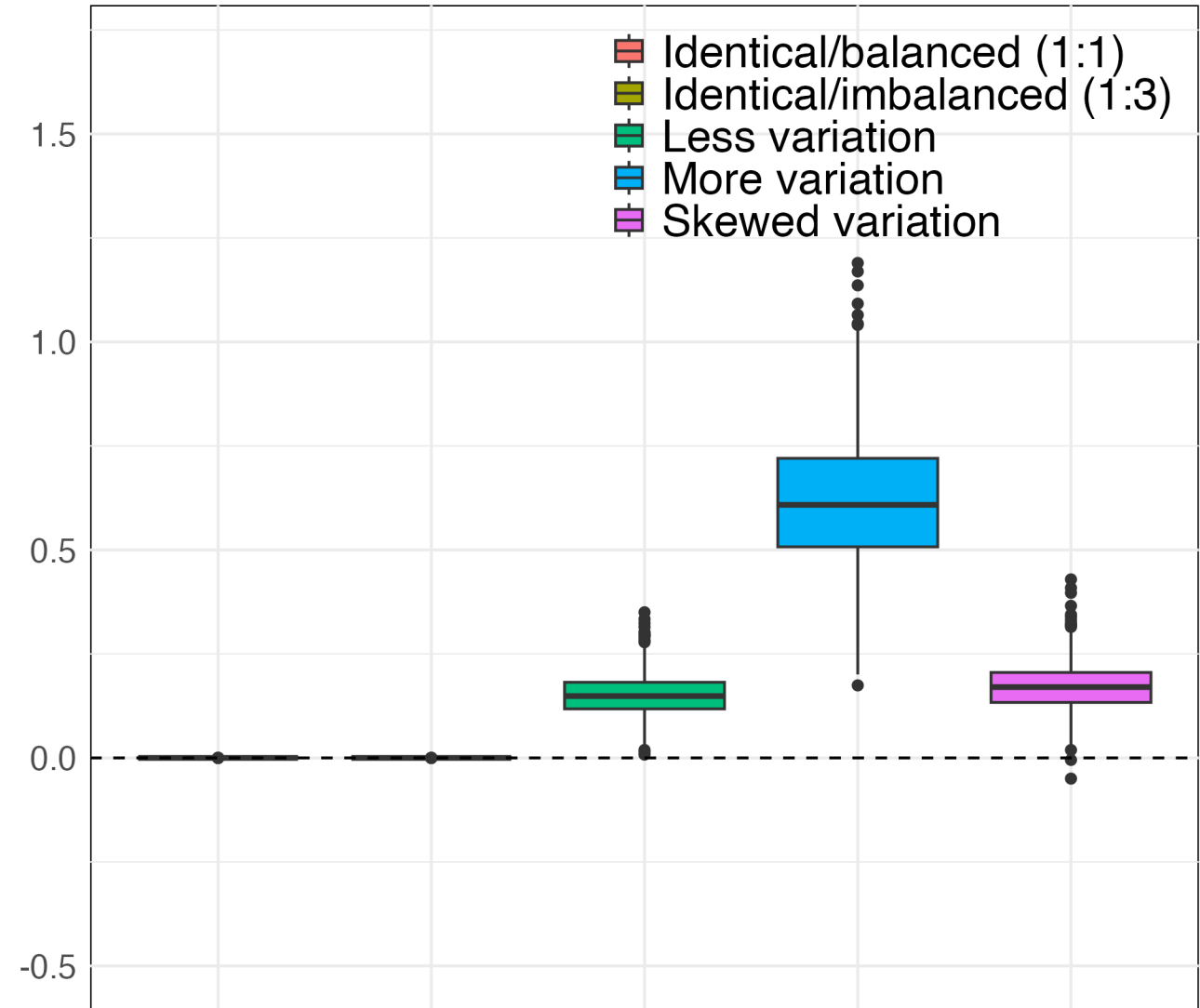
Noncollapsibility with confounding (aggregation bias)
