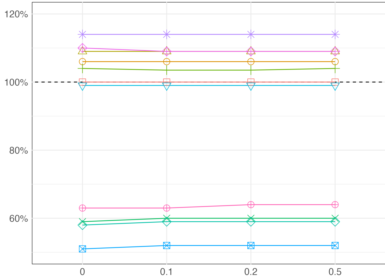
Noncollapsibility with confounding (aggregation bias)
