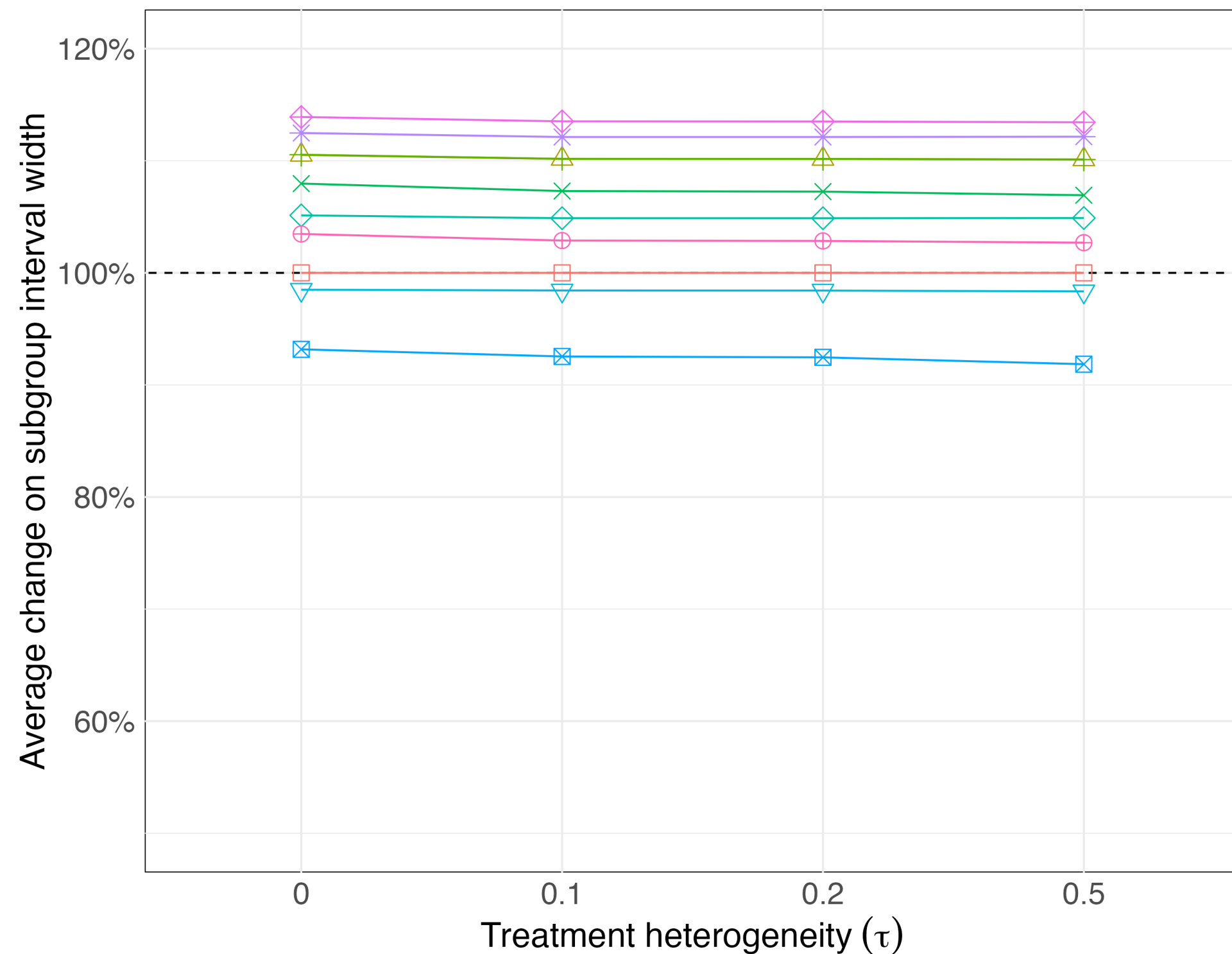
Noncollapsibility without confounding (no aggregation bias)
