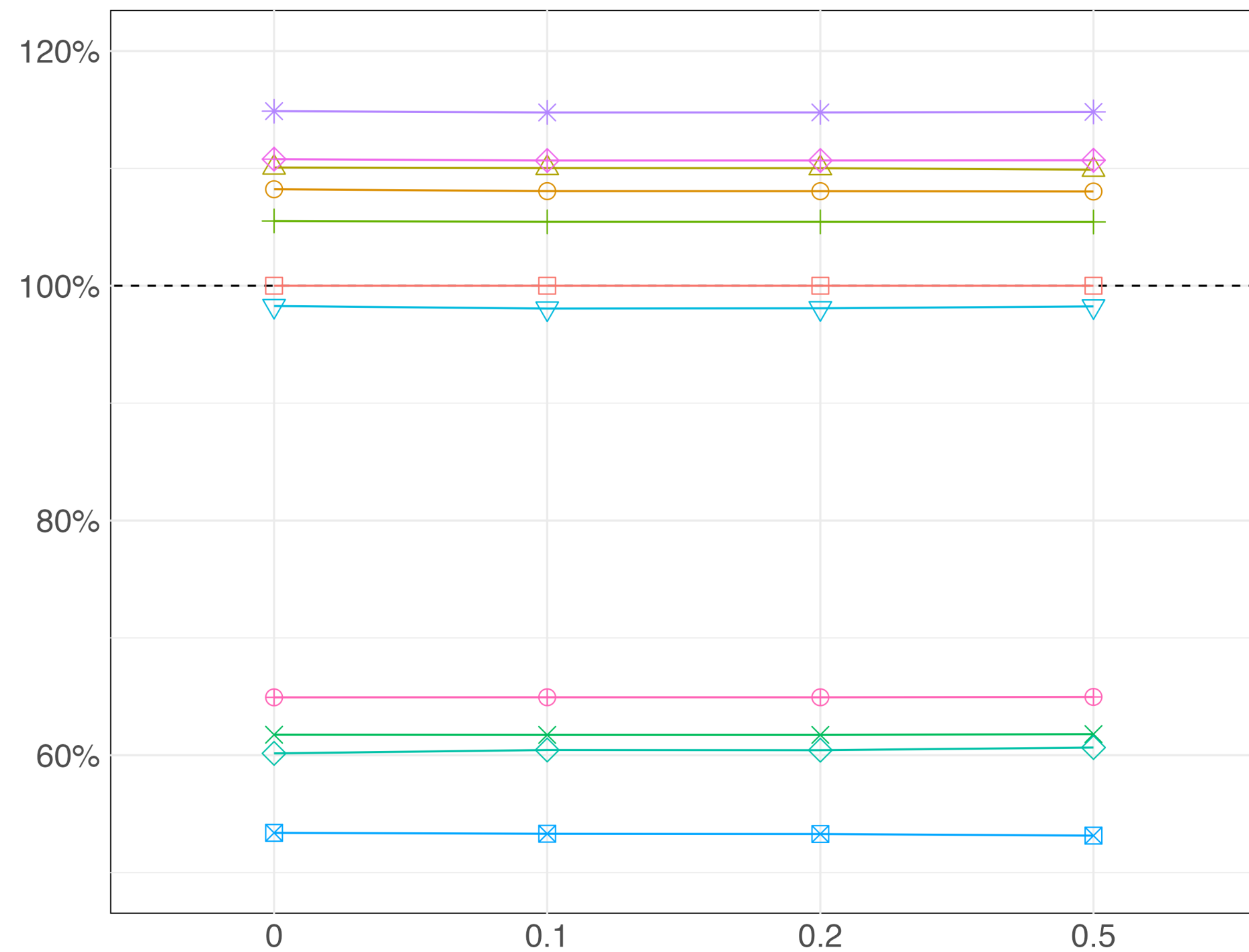
Noncollapsibility with confounding (aggregation bias)
