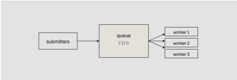
Fig. 7.1 Submitters push callables into a FIFO work queue; a fixed set of workers pull from it.
