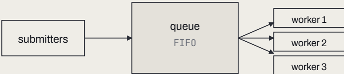
Fig. 1 Submitters push callables into a FIFO work queue; a fixed set of workers pull from it.
