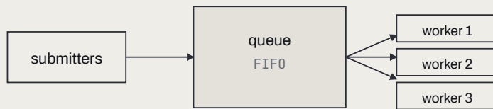
Fig. 1 Submitters push callables into a FIFO work queue; a fixed set of workers pull from it.
