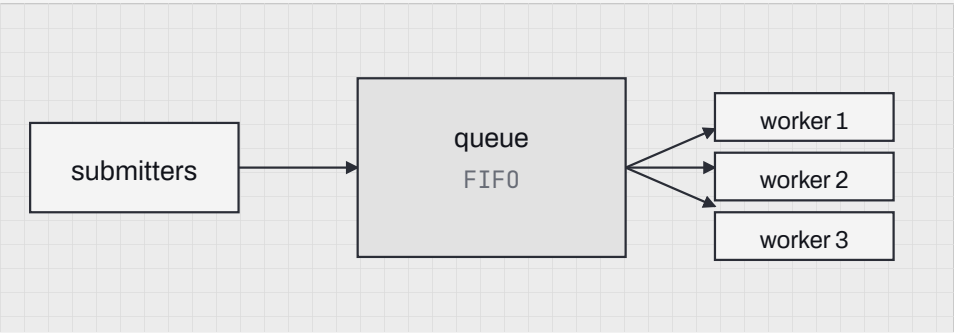
Fig. 7.1 Submitters push callables into a FIFO work queue; a fixed set of workers pull from it.
