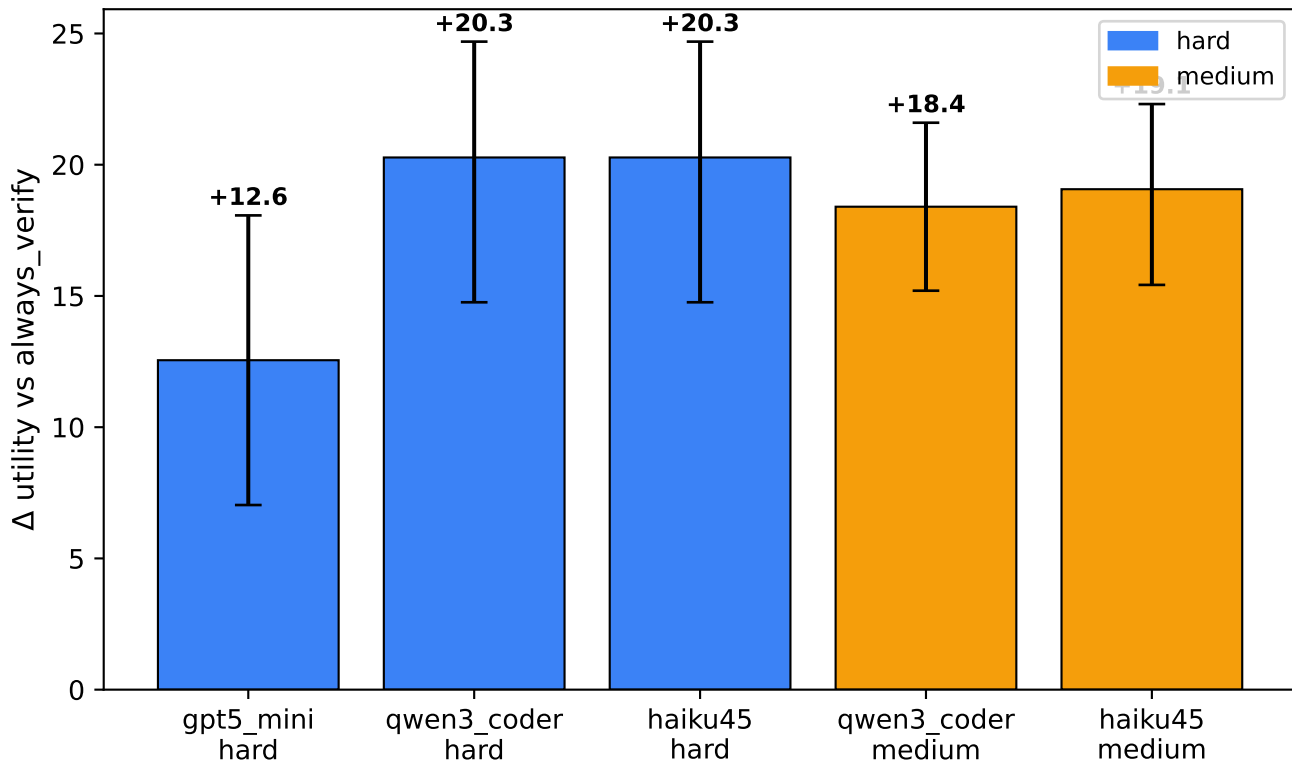
Bayesian Greedy: pre-registered effect, replicated across generators × difficulties
