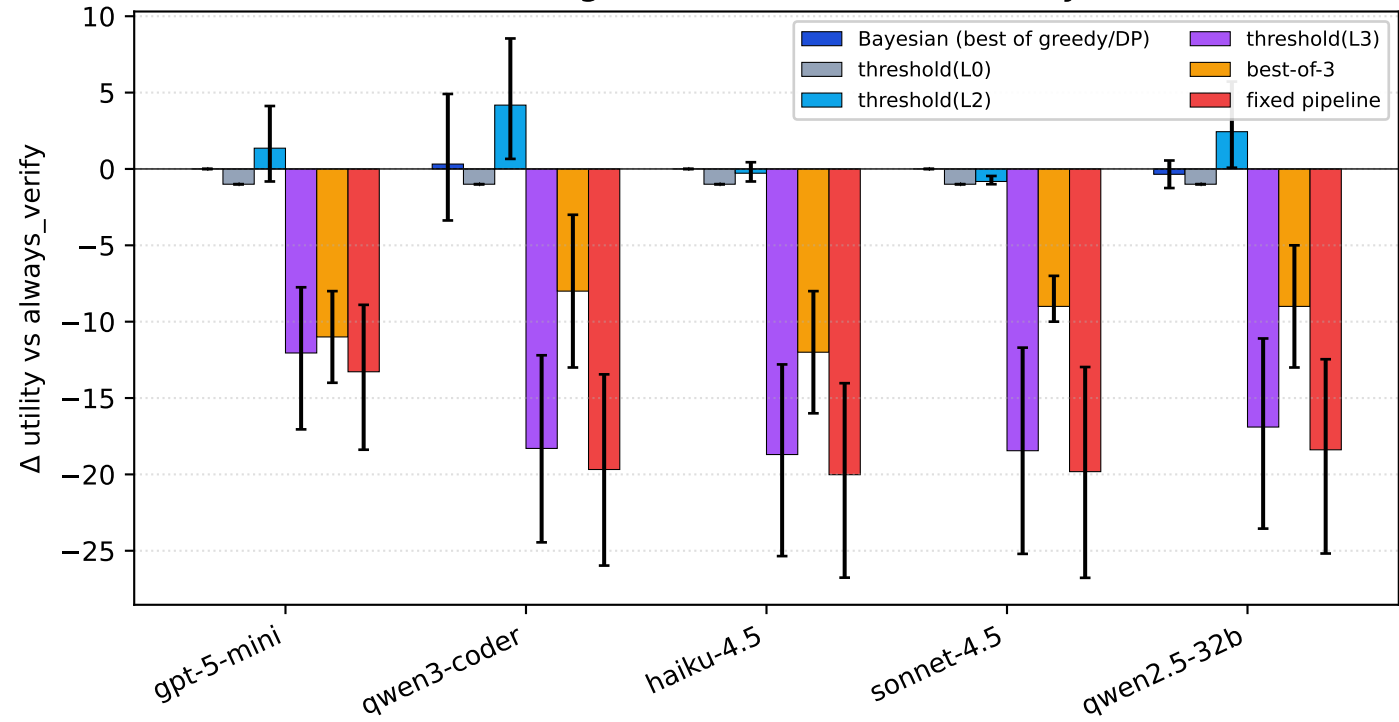
HumanEval+ (regime C: saturated, no iter trajectories)
