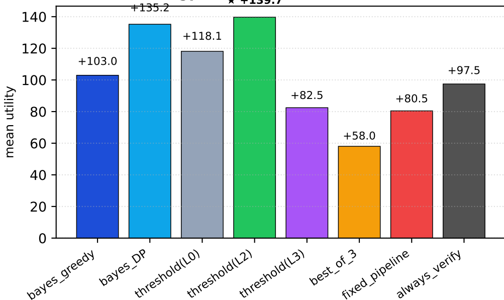
lcb hard / gpt-5-mini (API) ( R = 500 , c_{\text{ver}} = 30 )
