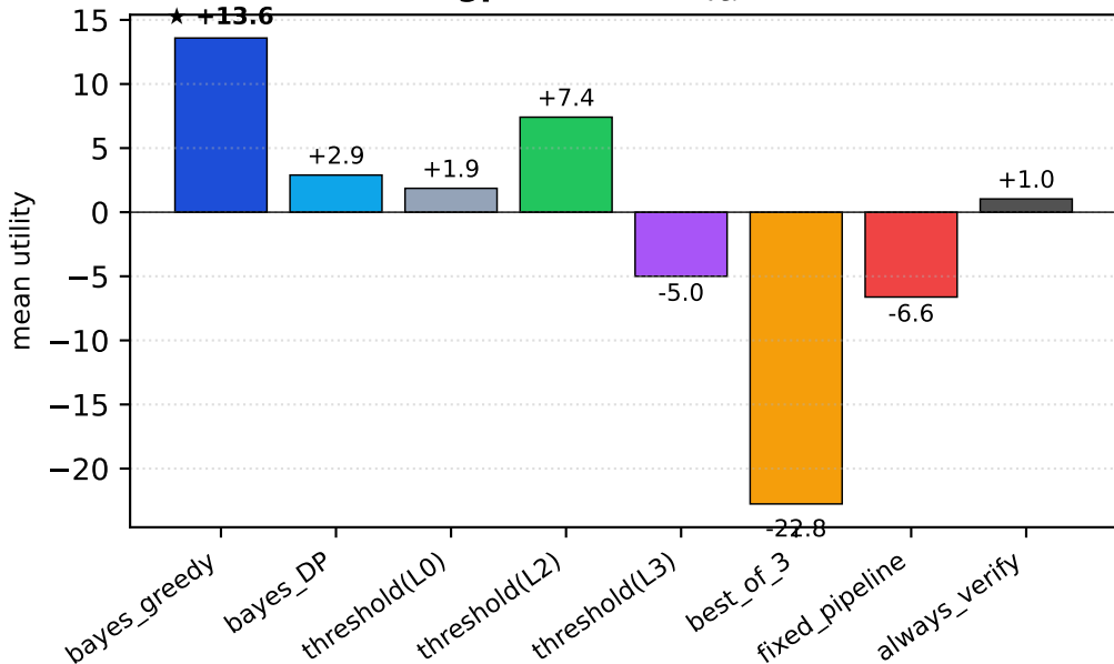
LCB-hard / gpt-5-mini ( c_{\text{ver}} = 30 , R = 100 )
