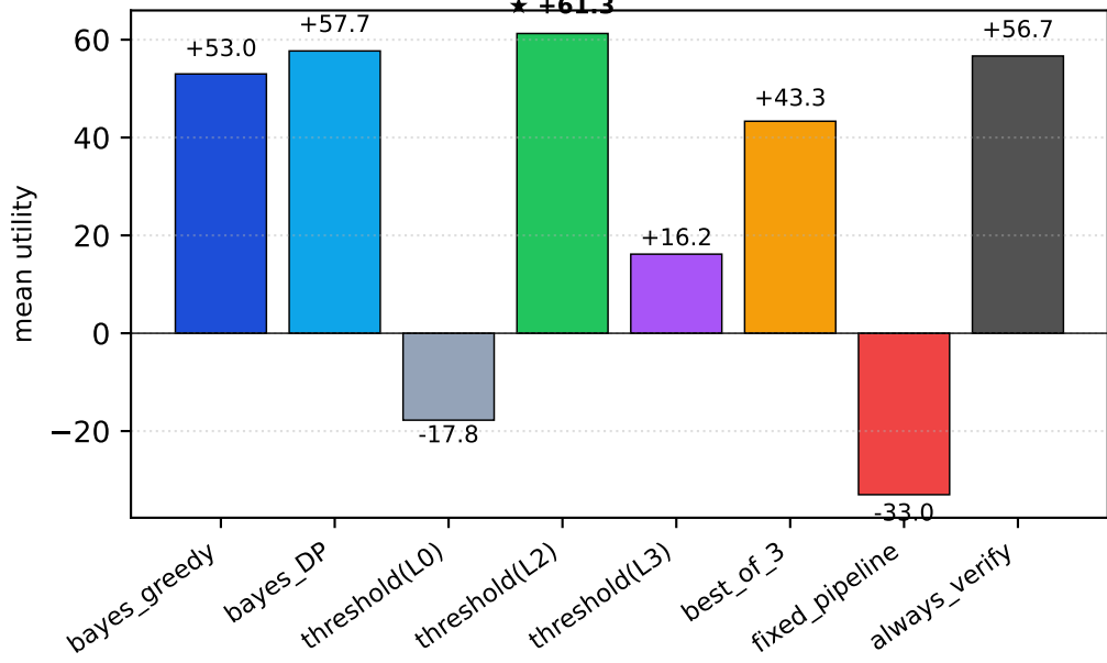
swe verified / sonnet-4.5 (API) ( c_{\text{ver}} = 10 , R = 100 )
