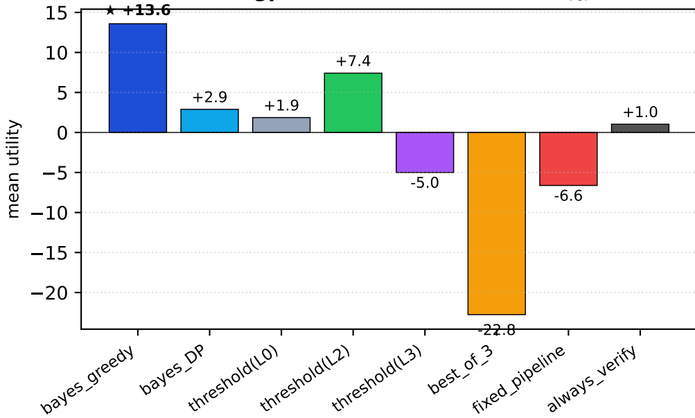
LCB-hard / gpt-5-mini (API) ( R = 100 , c_{\text{ver}} = 30 )
