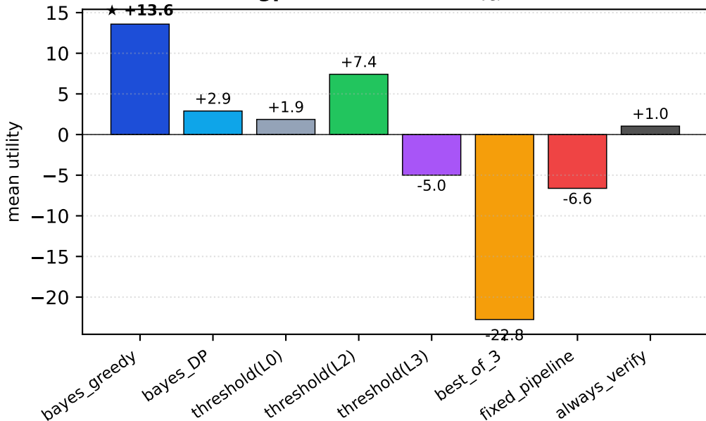
LCB-hard / gpt-5-mini (API) ( c_{\text{ver}} = 30, R = 100 )
