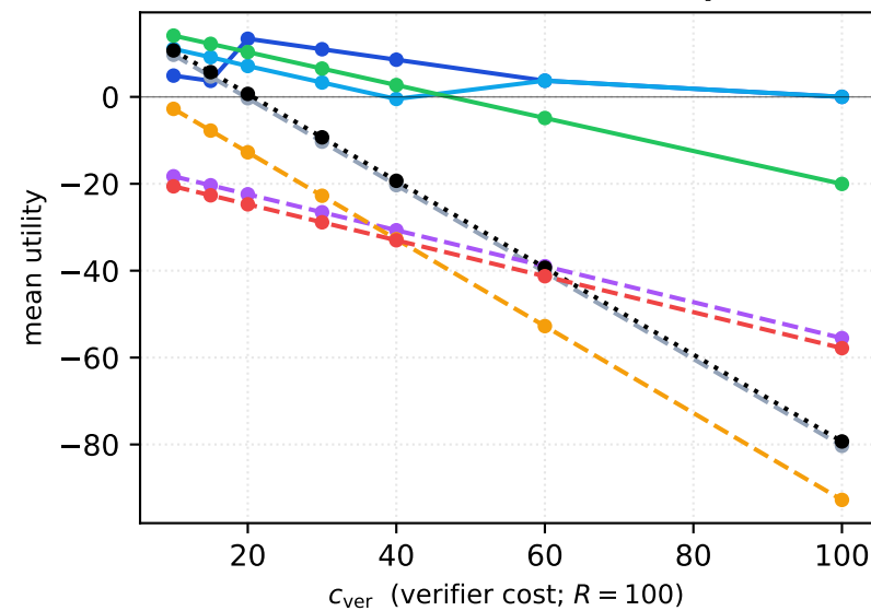
sonnet-4.5 (API) (LCB-hard, n=29, prior=0.20)
