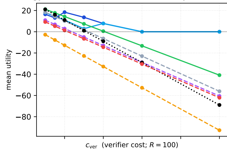
gpt-5-mini (API) (LCB-hard, n=29, prior=0.25)
