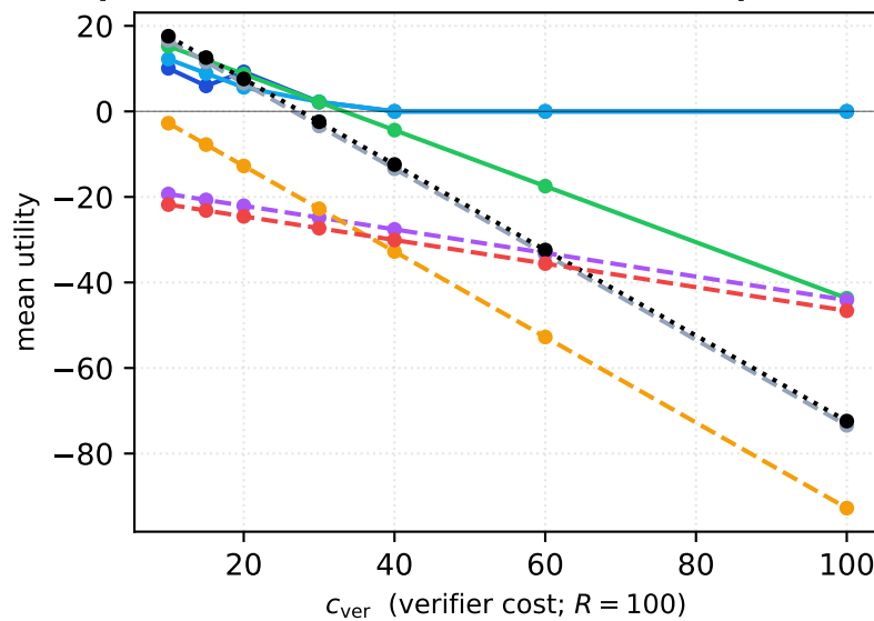
qwen2.5-32b (local) (LCB-hard, n=29, prior=0.21)
