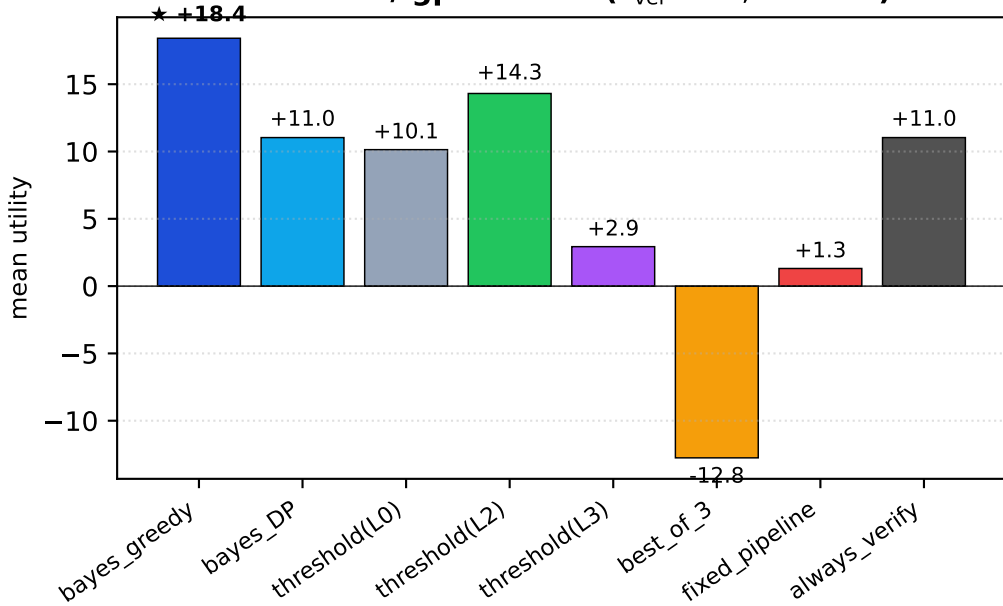
LCB-hard / gpt-5-mini ( c_{\text{ver}} = 20 , R = 100 )
