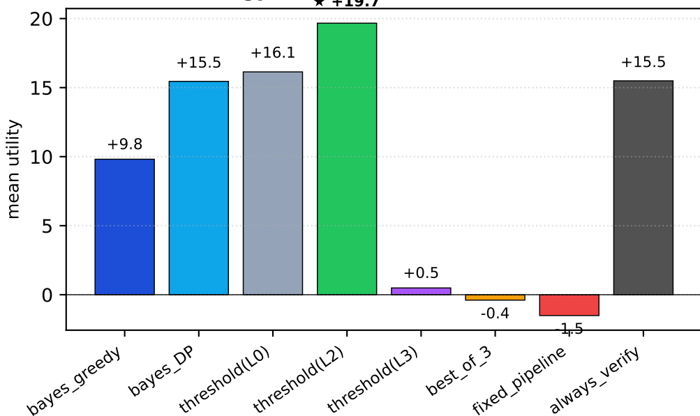
lcb hard / gpt-5-mini (API) ( C_{\text{ver}} = 10 , R = 100 )
