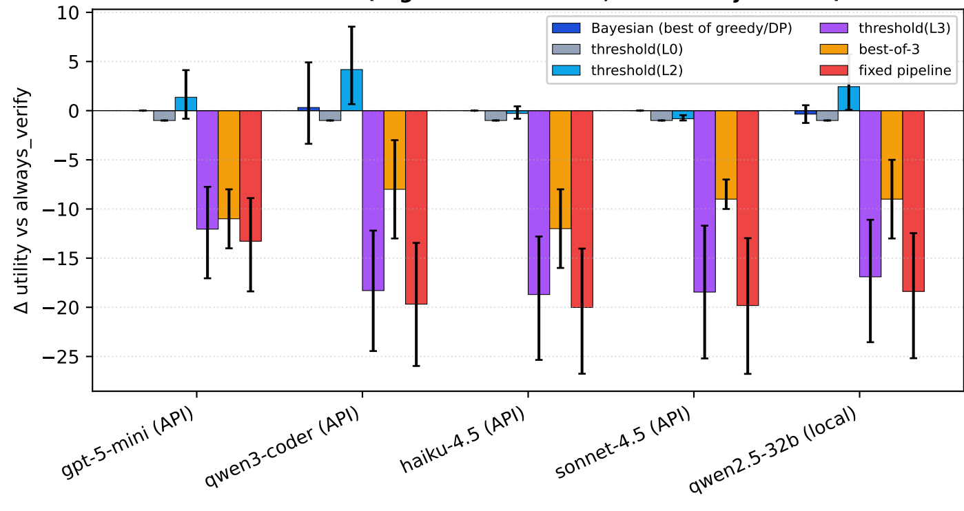
HumanEval+ (regime C: saturated, no iter trajectories)
