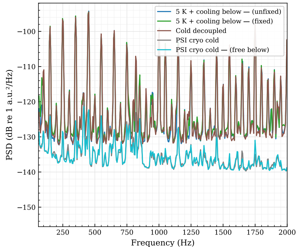
Welch PSD — linear freq. axis
