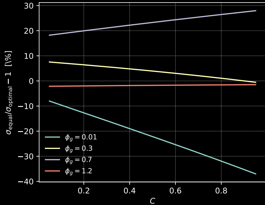
Gain of optimal over equal 120° spacing
