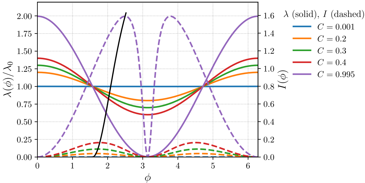
Mean photon number \lambda(\phi) and Fisher information I(\phi) for a displaced thermal state as a function of phase \phi
