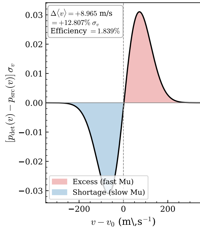
(c) Lifetime-induced redistribution
