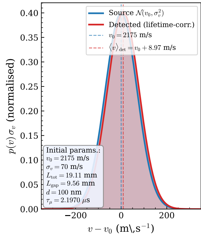
(a) Velocity distributions
