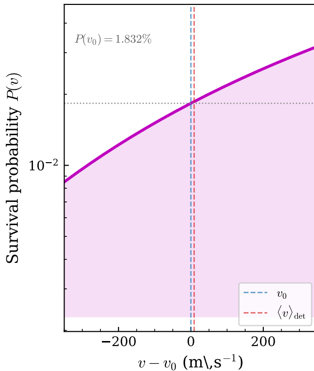
(b) Muon survival \exp(-L_{\text{tot}}/v\tau)
