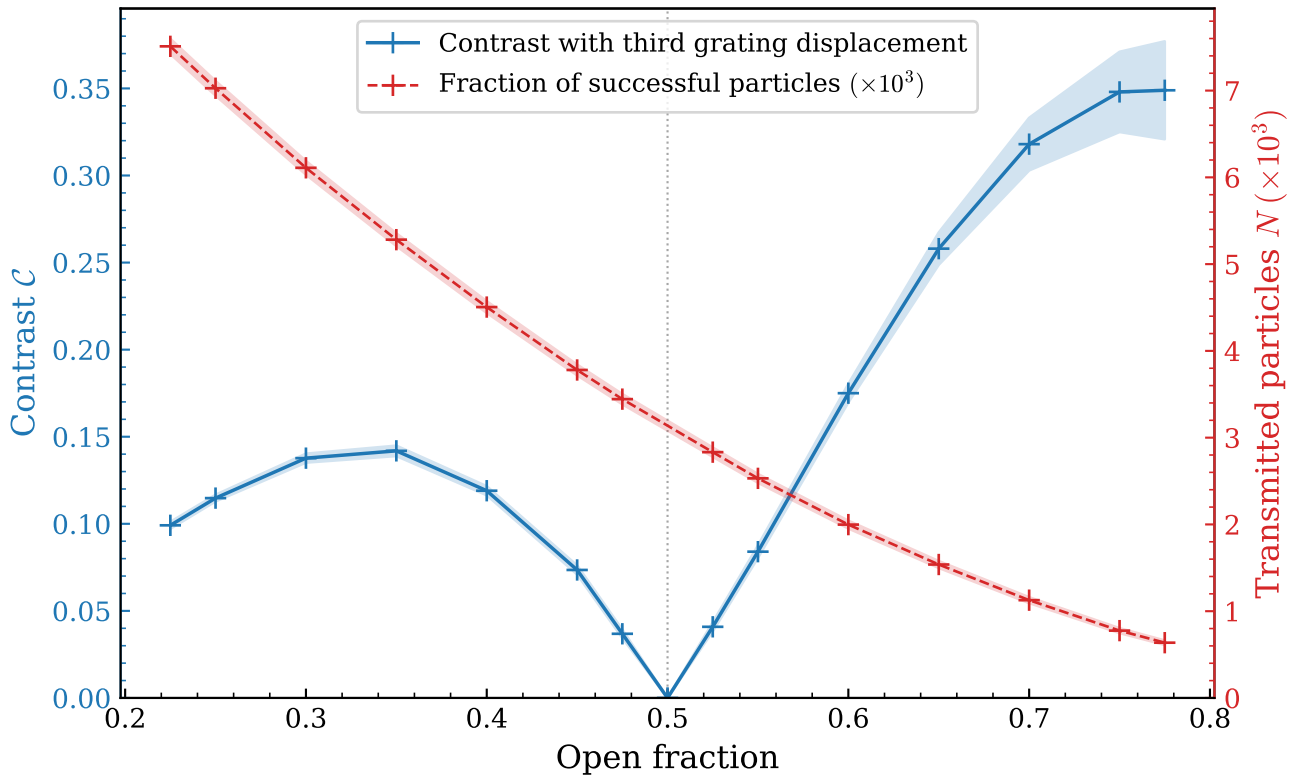
Classical simulation: contrast and transmission vs. duty cycle
