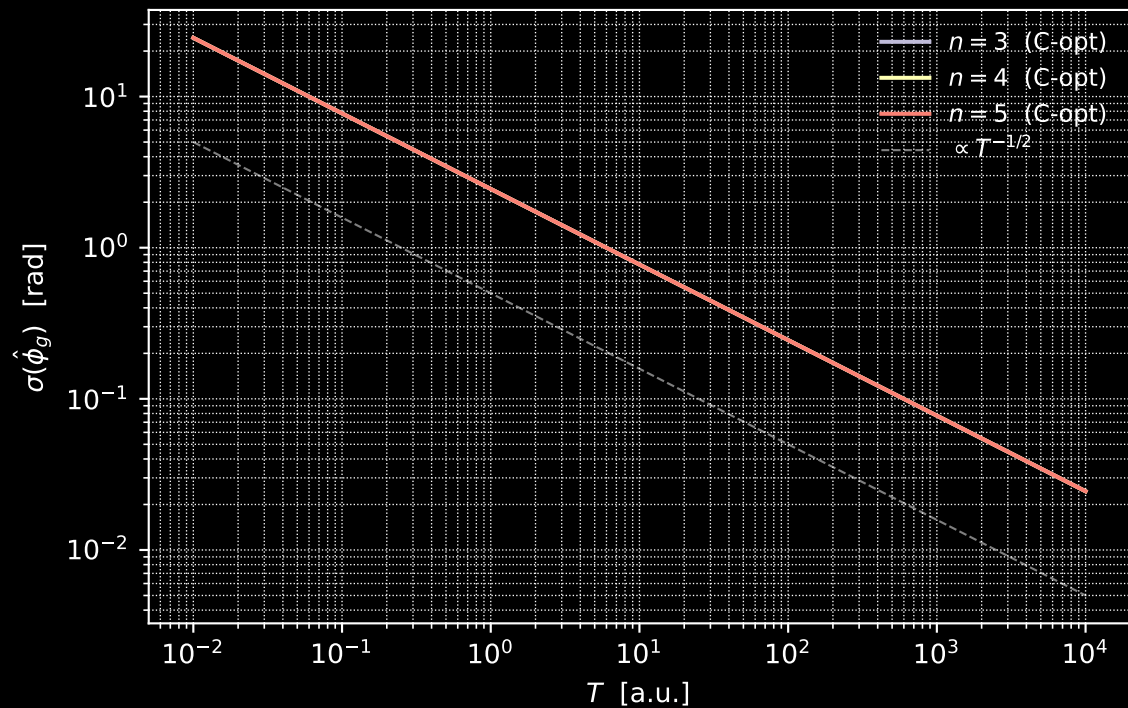
Precision vs total time
