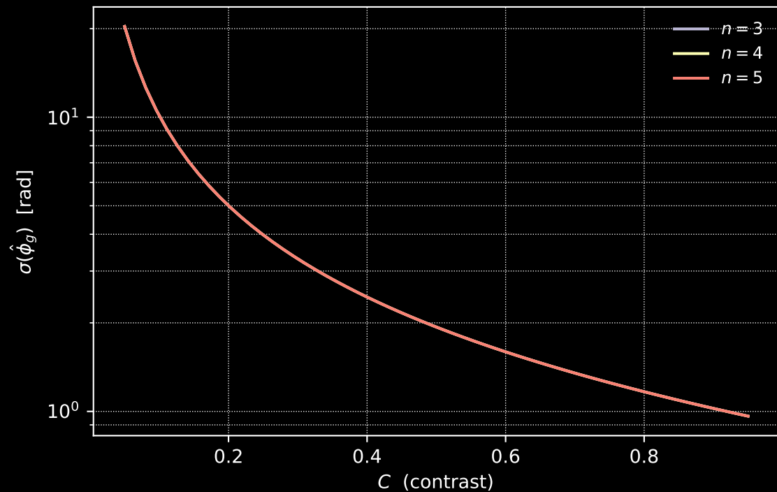
Precision vs contrast (positions fixed at C = 0.4 optimum)
