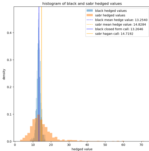
Figure: Strike K = 751.0
