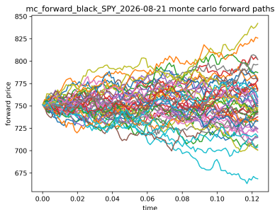
(a) Black model forward paths.
