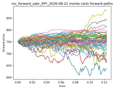
(b) SABR model forward paths.
