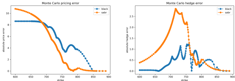
Figure: Comparison of the Monte Carlo pricing error and dynamic hedging error for the Black and SABR models across different strike prices. The left panel shows the absolute pricing error between the Monte Carlo estimate and the corresponding closed form option price, while the right panel shows the absolute hedging error obtained from the dynamic delta hedging simulation.
