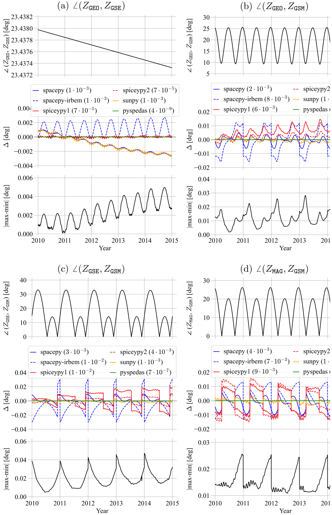
Figure 3: Angles between Z axes in select coordinate frames as computed by different software packages. In the top panels of each subplot, the notation \angle(Z_A, Z_B) means the angle between the Z axis of coordinate frame A and the Z axis of coordinate frame B computed using geopack_08_dp . The middle panel of each subplot shows the difference \Delta , between \angle(Z_A, Z_B) computed using geopack_08_dp and that computed using the library indicated in the legend; the maximum of the absolute value of each line is shown in parentheses. The bottom panels show the maximum absolute differences in the middle panel.
