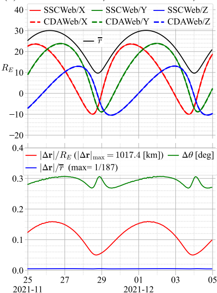
(a) Geotail SSCWeb/GEI vs. CDAWeb/GEI
