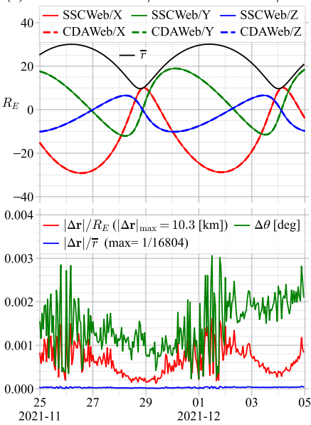
(c) Geotail SSCWeb/GSE vs. CDAWeb/GSE
