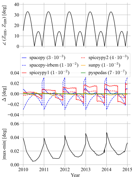
(c) \angle(Z_{\text{GSE}}, Z_{\text{GSM}})
