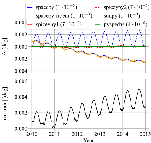
(c) \angle(Z_{\text{GSE}}, Z_{\text{GSM}})
