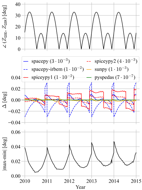
(c) \angle(Z_{\text{GSE}}, Z_{\text{GSM}})
