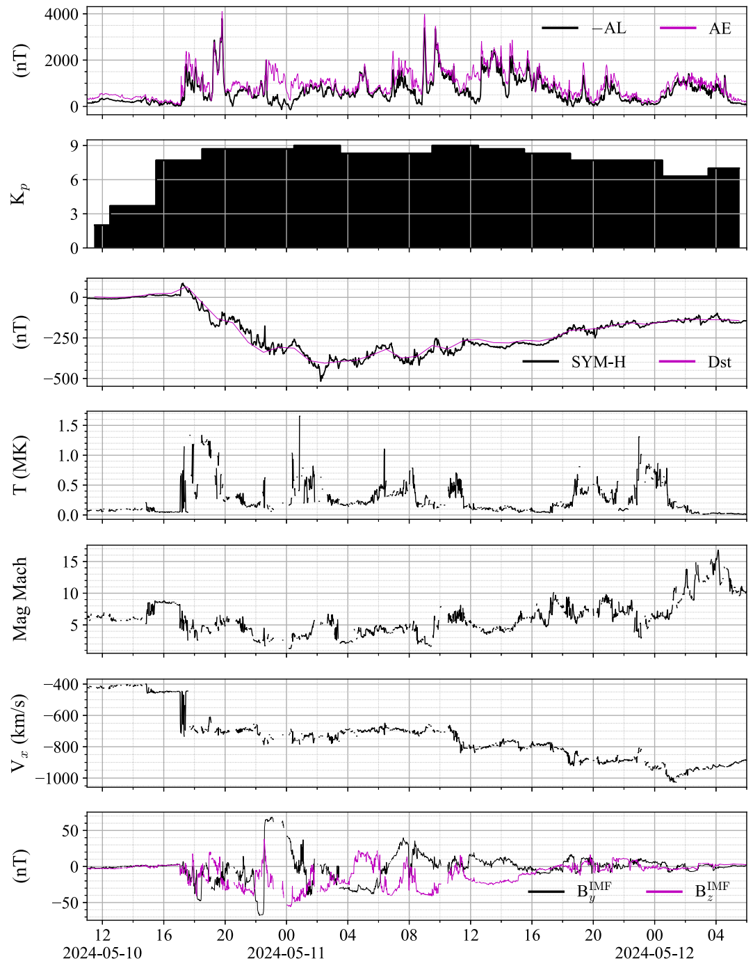
Figure 1. Solar wind conditions and select geomagnetic indices during the May 2024 storm event from the OMNI data set (Papitashvili and King (2020b); Papitashvili and King (2020a)) using the HAPI (Weigel et al., 2021) server. AE is the Auroral Electrojet index, and AL is the Auroral Electrojet index, Lower. The K p index is based on the surface B field variation over 3 hr intervals, with values ranging from 0 to 9. The SYM-H index, related to Dst, is a measure of the deviation of the horizontal (H) component of the B field. T is the temperature of the proton component of the thermal solar wind. Mag Mach (magnetosonic Mach number) is a dimensionless quantity representing the ratio of the solar wind velocity to the local Alfvén speed. V x is the x component of the solar wind velocity. B y IMF and B z IMF are the B field components of the IMF in the y and z directions, respectively.
