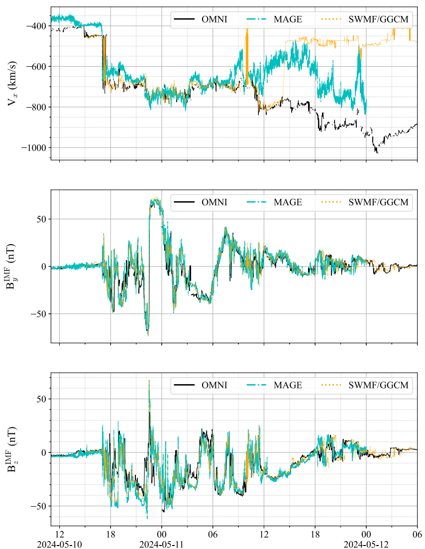
Figure A1. Comparison of V_x , B_y^{\text{IMF}} , and B_z^{\text{IMF}} used as inputs for the different geospace environment models (Multiscale Atmosphere-Geospace Environment Model, Space Weather Modeling Framework, Open Geospace General Circulation Model) as discussed in Section 2.4. OMNI data is the same as that presented in Figure 1.
