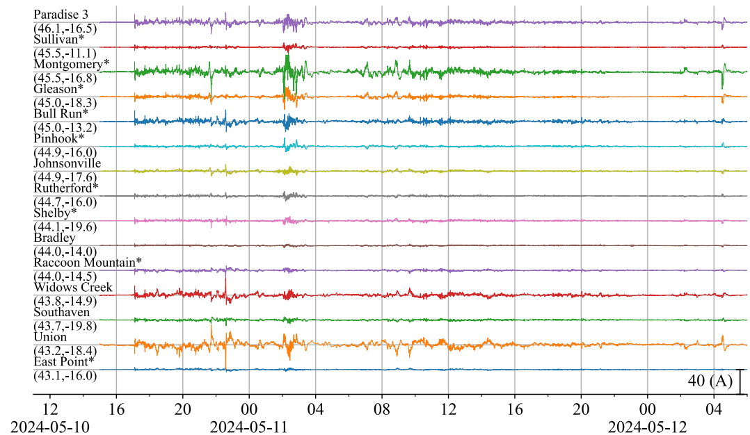
Figure 3. Geomagnetically induced current times series from 15 Tennessee Valley Authority sites shown with 40 A baseline offsets, sorted by geomagnetic latitude, and labeled with the site name and its geomagnetic latitude and longitude in degrees. Data from nine sites that were also found in the North American Electric Reliability Corporation database are indicated with an asterisk.
