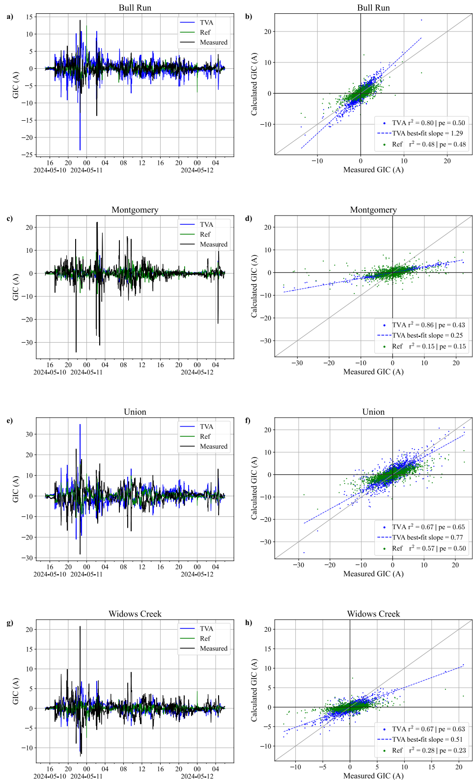
Figure 6. Measured Geomagnetically induced current, Tennessee Valley Authority model, and Reference model timeseries (left) and scatter correlation plots (right).
