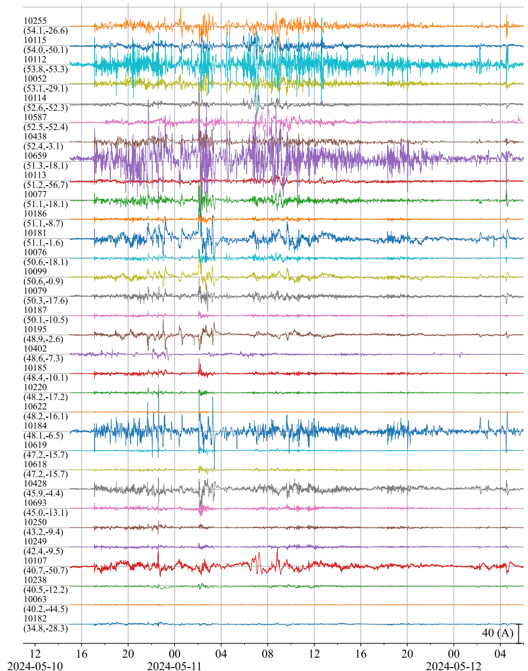
Figure 4. Geomagnetically induced current (GIC) data from 32 sites from NERC's Electric Reliability Organization portal with 40 A baseline offsets sorted by geomagnetic latitude and labeled with the North American Electric Reliability Corporation (NERC) site ID and its geomagnetic latitude and longitude in degrees. All NERC GIC data were either measured from a three-phase transformer or scaled to be equivalent.
