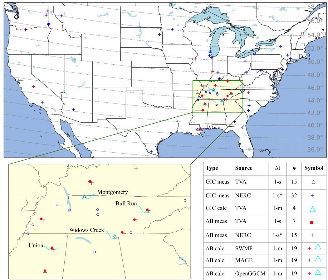
Figure 2. Geomagnetically induced current (GIC) and magnetometer (measured difference in the surface magnetic field from a baseline, or \Delta B ) locations and locations where model estimates are available. The approximate Tennessee Valley Authority operating region is shown in the yellow box. The inset table describes the measurement type, measurement source, cadence ( \Delta t ), and number of sites (#) for each symbol. *Note that \Delta t for North American Electric Reliability Corporation GIC and \Delta B measured sites varied, with GIC sites having cadences of 1 s, 2 s, 4 s, 5 s, 1 min, 5 min, and 1 hr and \Delta B sites having cadences of 1 s, 10 s, and 1 min.
