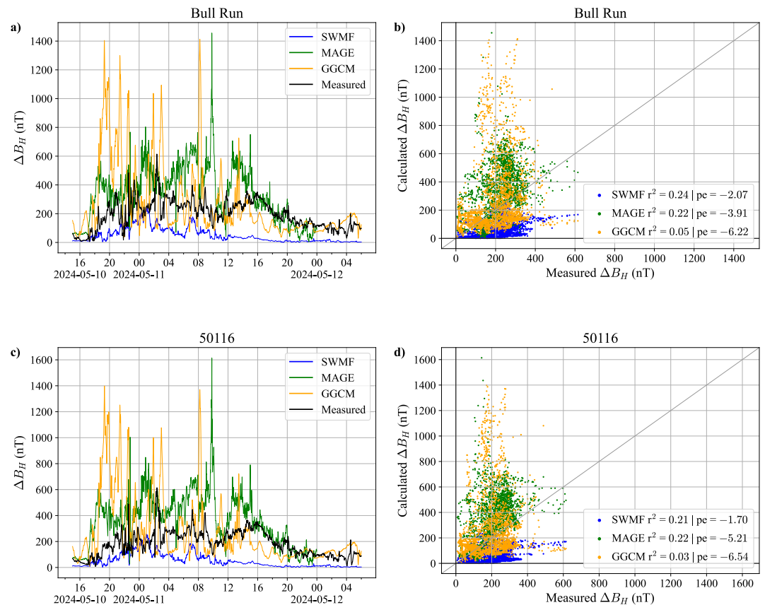
Figure 7. Calculated (Space Weather Modeling Framework, Multiscale Atmosphere-Geospace Environment Model, and Open Geospace General Circulation Model) and measured \Delta B_H timeseries comparison (left) and scatter correlation plots (right).
