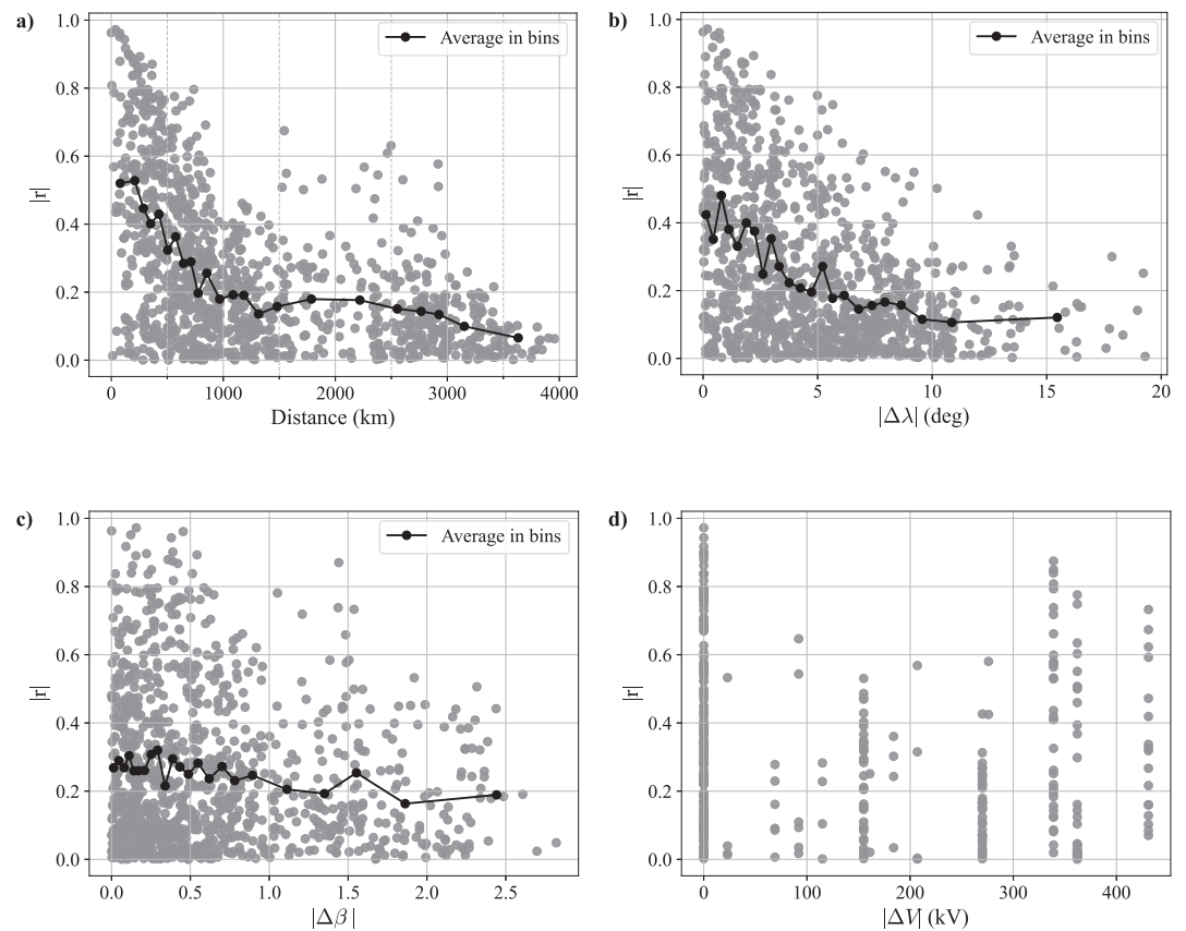
Figure 8. Correlation between Geomagnetically induced current (GIC) timeseries for 1,081 site pairs (except for \Delta V shown in subplot (d), which was only available for 325 of the 1,081 site pairs) vs. (a) differences in site pair separation distance, (b) geomagnetic latitude ( \lambda ), (c) conductivity scaling factor ( \beta ), and (d) power line voltage nearest to the GIC instrument. Mean |r| values are shown as black dots centered on 23 bins with 47 points in each bin.
