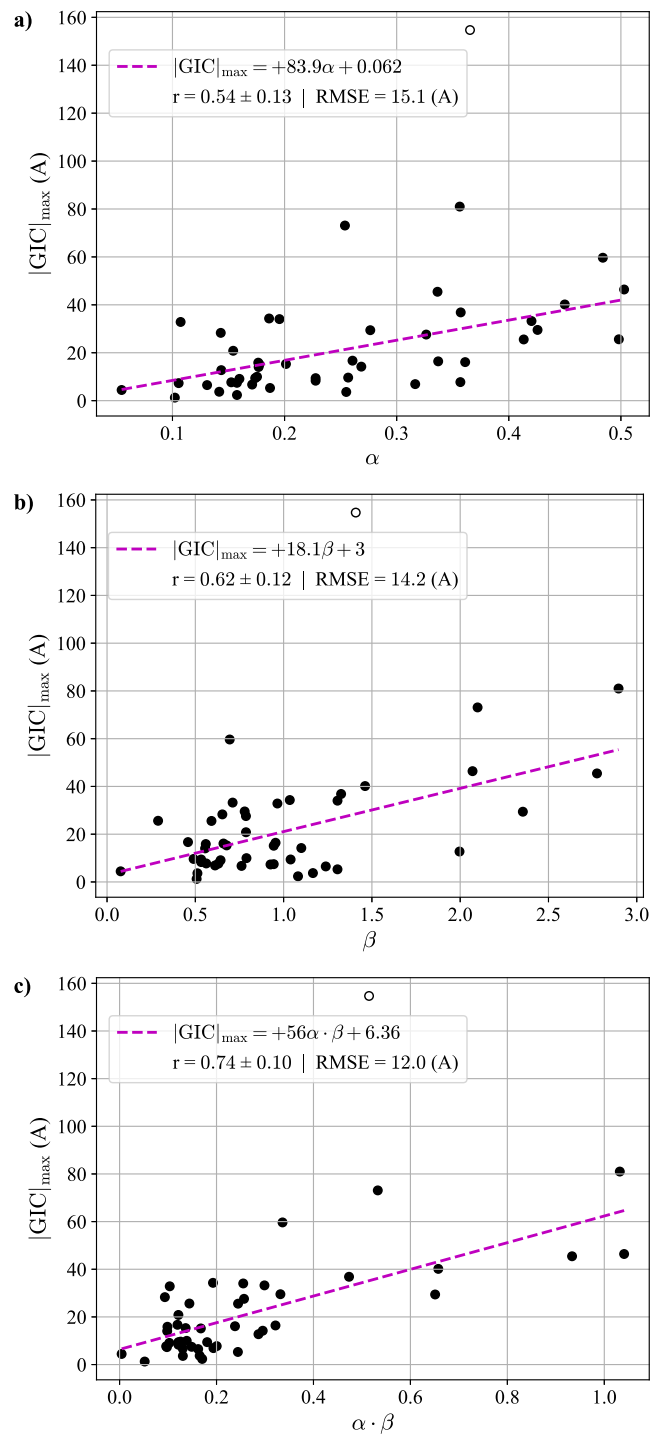
Figure 10. Geomagnetically induced current linear regression relationships. The white circle is an outlier that was excluded from the calculation of model parameters.
