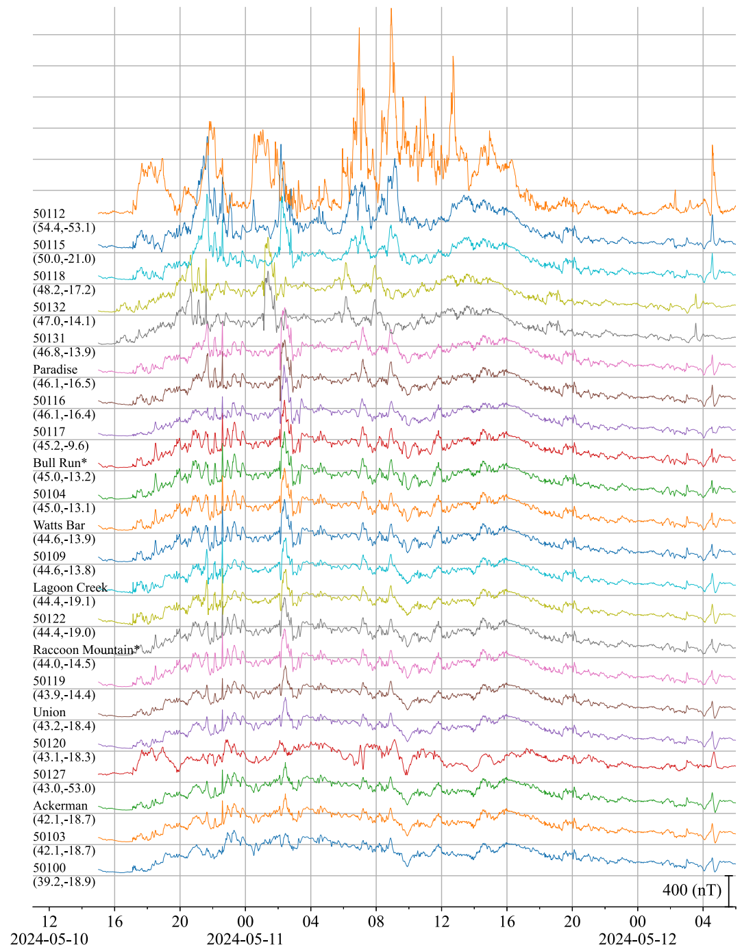
Figure 5. \Delta B_H measurements from 15 sites from NERC's Electric Reliability Organization portal and 7 sites from Tennessee Valley Authority with 400 nT baseline offsets sorted by geomagnetic latitude and labeled with the site ID and its geomagnetic latitude and longitude in degrees.
