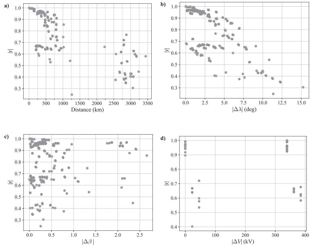
Figure 9. Same as Figure 8 except for \Delta B_H timeseries for all 231 magnetometer site pairs.
