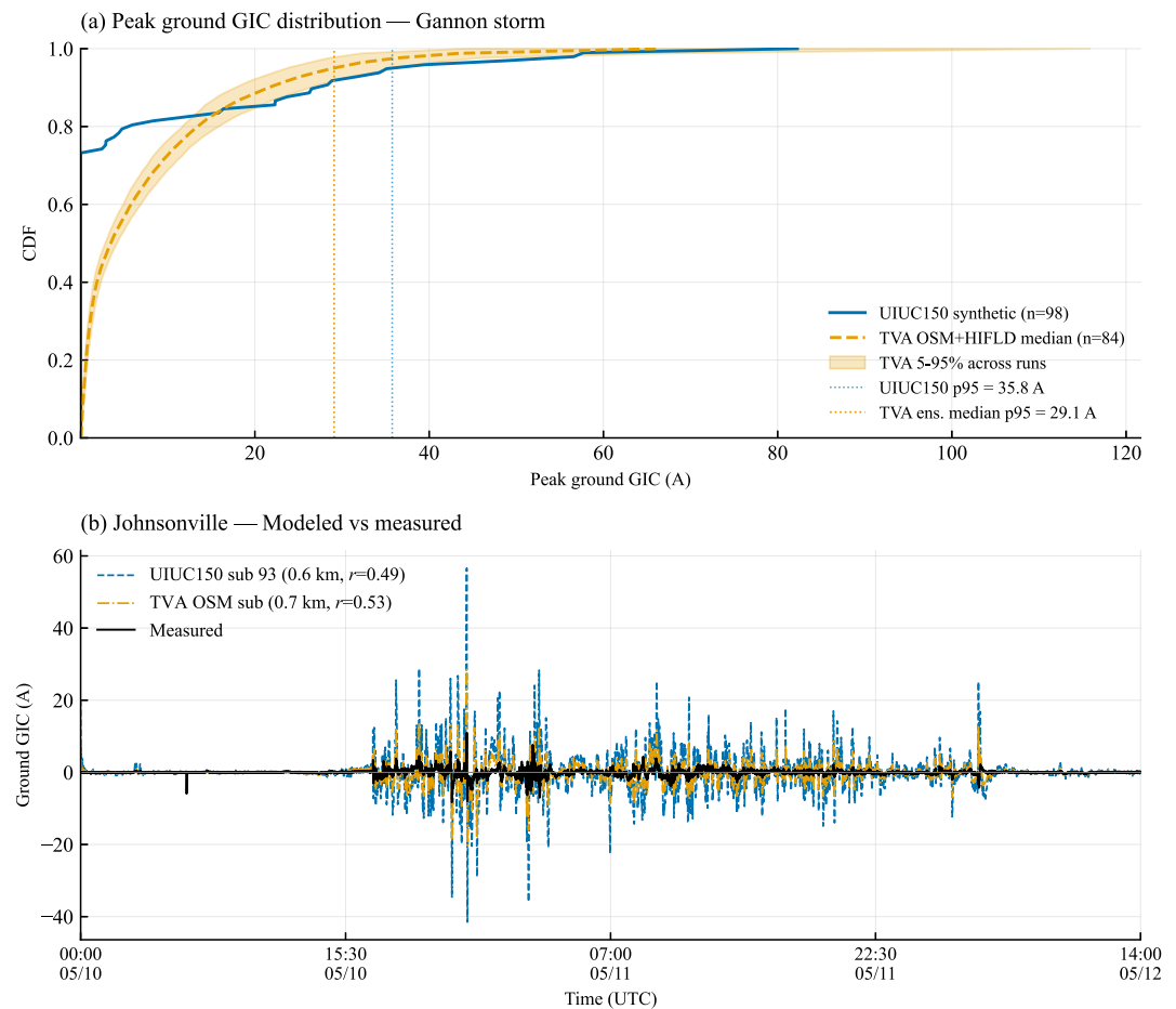
Figure 7. Comparison of modeled ground GIC between the UIUC150 synthetic network and the TVA OSM + HIFLD geospatial network during the May 2024 Gannon storm. Panel (a) shows the cumulative distribution of peak ground GIC. For the TVA OSM + HIFLD network, the median distribution across the Monte Carlo ensemble is shown with a shaded 5th to 95th percentile band, and the vertical dotted line marks the ensemble median 95th percentile (29.1 A). The UIUC150 synthetic network uses fixed published parameters, and its 95th percentile (35.8 A) is shown for comparison. Panel (b) shows modeled ground GIC time series at Johnsonville from both networks alongside TVA measurements, for the nearest UIUC150 substation at 0.6 km and the nearest OSM substation at 0.7 km separation distance.
