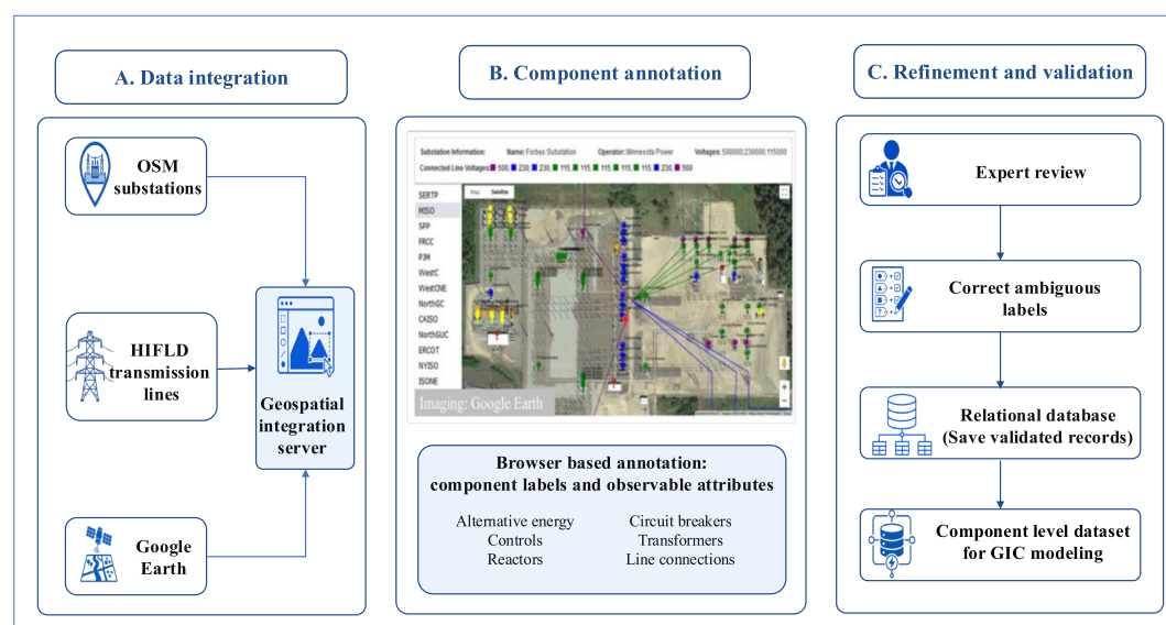
Figure 1. Overview of the methodology for identifying and mapping transmission assets for GIC assessment. (a) Data integration combines OpenStreetMap substations, Homeland Infrastructure Foundation-Level Data (HIFLD) transmission lines, and Google Earth imagery in a geospatial integration server. (b) Component annotation is made using a browser-based interface to label components and their observable attributes. (c) Refinement and validation applies expert review to correct ambiguous labels and stores validated records, yielding the component-level data set for GIC modeling.
