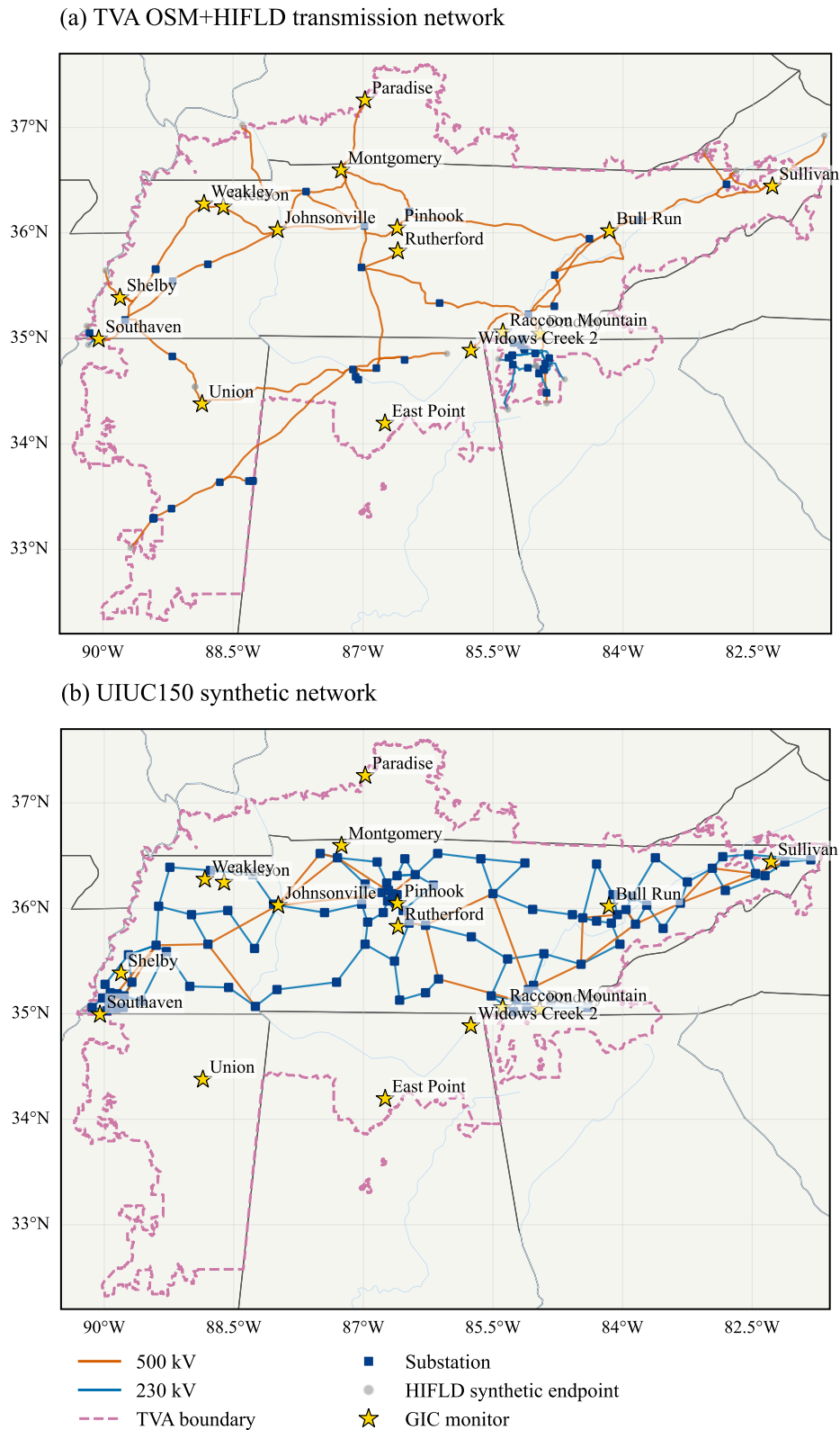
Figure 4. Two-panel map showing the TVA OSM + HIFLD backbone network (top) and the UIUC150 synthetic network (bottom), with the TVA service boundary, monitored substations, and GIC monitoring devices. The UIUC150 network is a synthetic grid statistically matched to regional load and generation, whereas the OSM + HIFLD network is built from open-source geospatial data on substation locations and the geometry of transmission lines.
