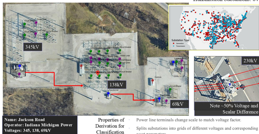
Figure 2. Voltage mapping by spatial configuration. Satellite imagery of Jackson Road substation (Indiana Michigan Power) showing component-level annotation across three voltage sections at 345, 138, and 69 kV. Annotated components include transformers, circuit breakers, power lines, and substation controls. The inset map shows the national distribution of 1,313 annotated substations classified as generation or transmission sites based on the presence and type of transformers identified.
