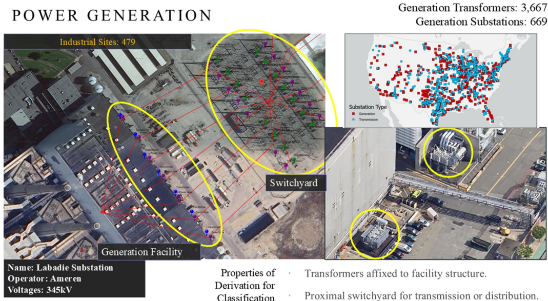
Figure 3. Refining areas of interest for specific component classes, such as generation transformers.
