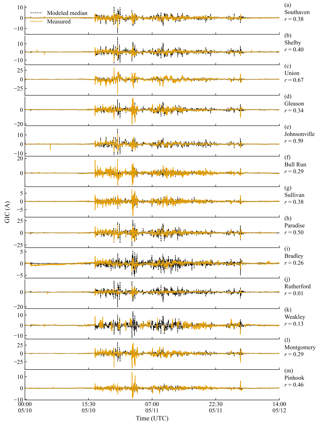
Figure 6. Time series comparison of modeled versus measured ground GIC at 13 TVA monitoring devices during the May 2024 Gannon storm. Each panel corresponds to one monitoring device, with the modeled ground GIC shown as the Monte Carlo ensemble median (dashed black line) and the measured GIC as a solid-colored line. The Pearson correlation coefficient between the modeled median and the measurement, together with the device identifier, is annotated for each site.
