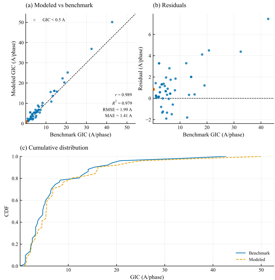
Figure 5. Comparison of modeled and benchmark effective GIC for 52 UIUC150 transformers under a uniform 1 V/km eastward geoelectric field. Panel (a) shows modeled versus benchmark effective GIC per transformer, with a 1:1 reference line. Panel (b) shows residuals as a function of benchmark GIC. Panel (c) shows the cumulative distribution of effective GIC for both the modeled and benchmark data sets, illustrating overall agreement in the distribution of GIC magnitudes across individual transformers.
