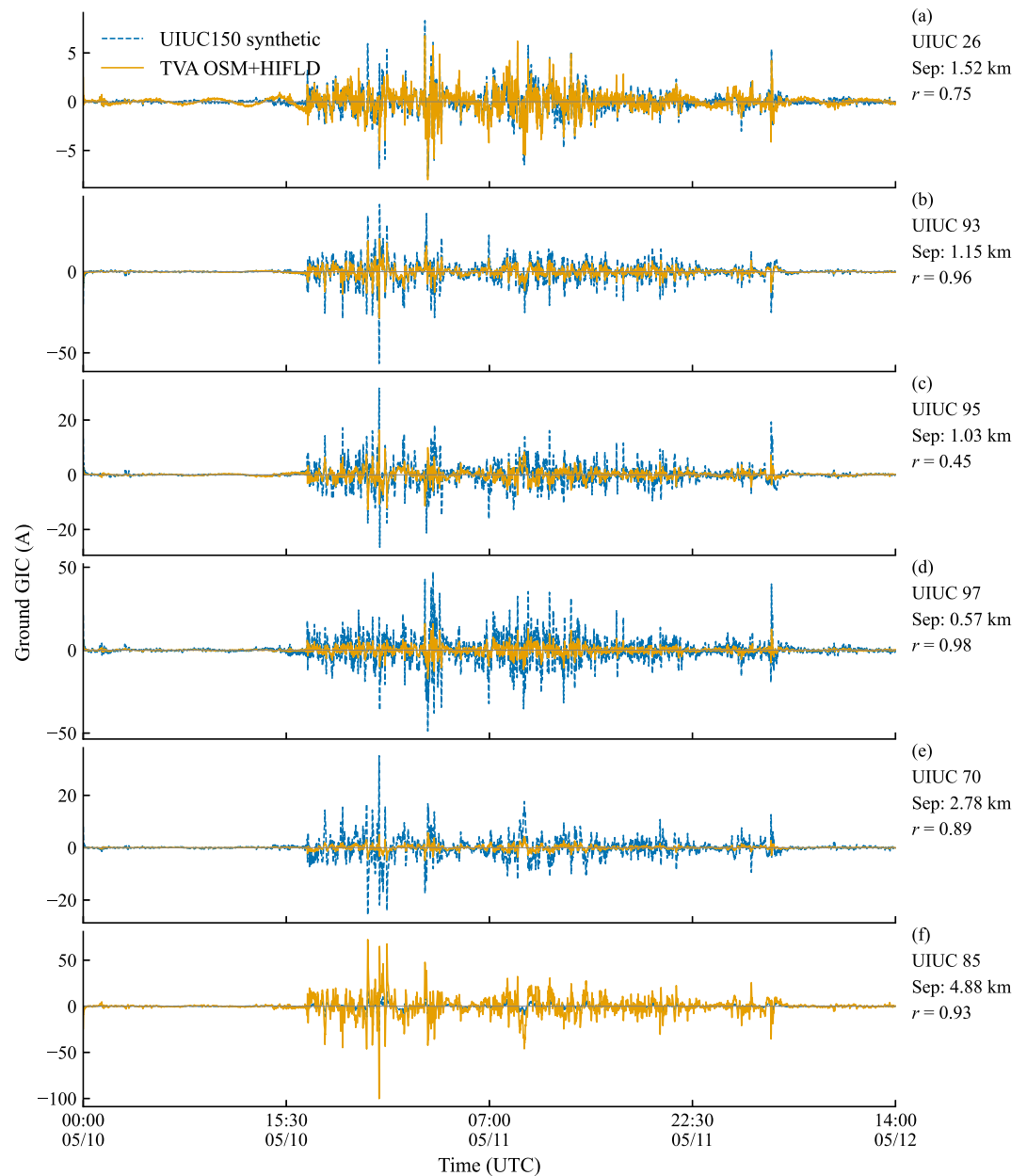
Figure 8. Modeled ground GIC at six matched UIUC150 synthetic and TVA OSM + HIFLD substation pairs during the May 2024 Gannon geomagnetic storm. Each panel corresponds to a matched pair, identified by the UIUC150 substation number and the separation distance (Sep.) between the two substations. The UIUC150-modeled GIC is shown as a dashed blue line, and the TVA OSM + HIFLD-modeled GIC as a solid orange line. Pearson correlation coefficients are computed over the full storm period shown. When the two networks produce negatively correlated time series, the sign of the UIUC150 values is corrected to align with the current reference directions, as noted in the relevant panels.
