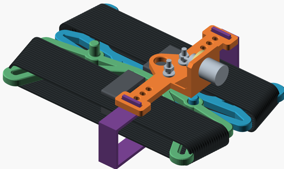
Separate coils. Compact center. Short rear strap. CAD packing illustration.
